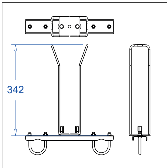
Snake extension 30 truss with stacking bracket
