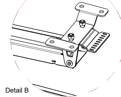
Snake ceiling mount
