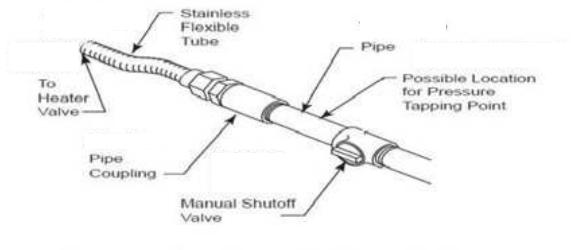
Typical components of a supply gas line, natural or propane
