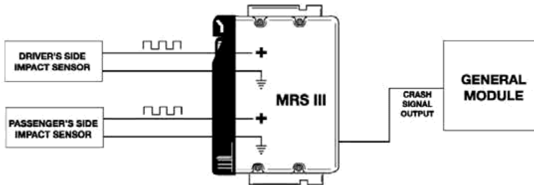
Fig. 3: Identifying Satellite Sensors Communication Diagram
