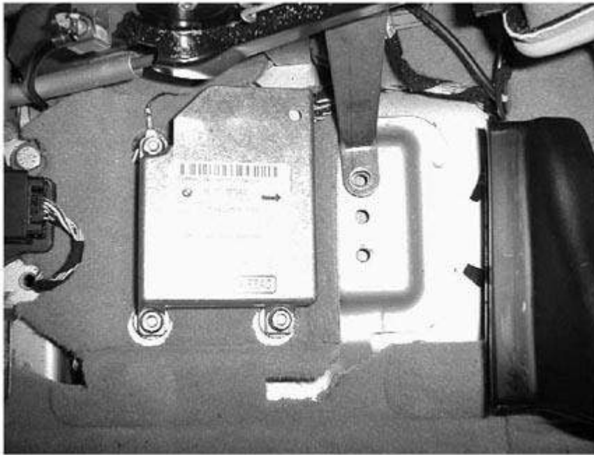
Fig. 1: Identifying MRS III Control Module Courtesy of BMW OF NORTH AMERICA, INC.
