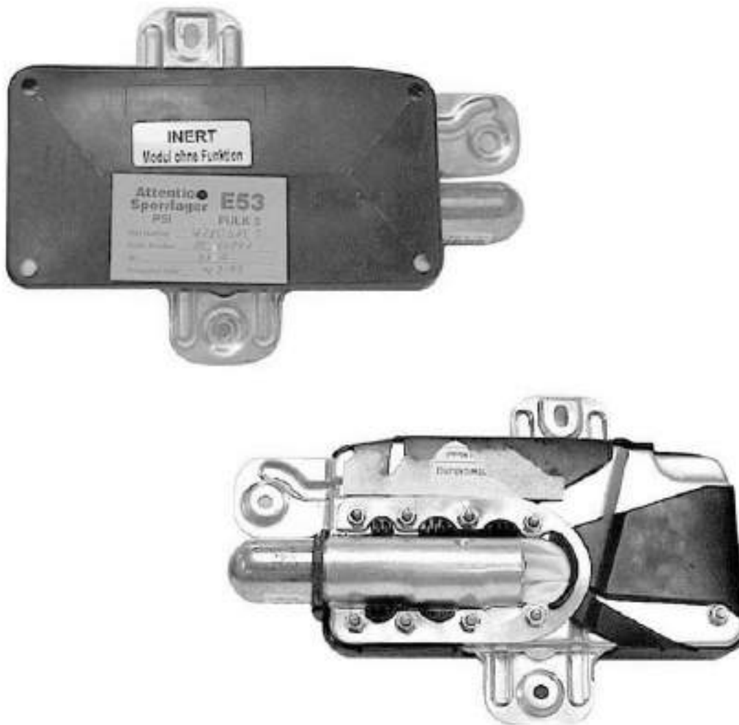
Fig. 7: Identifying Side Airbags Front/Rear (Thorax) Courtesy of BMW OF NORTH AMERICA, INC.
