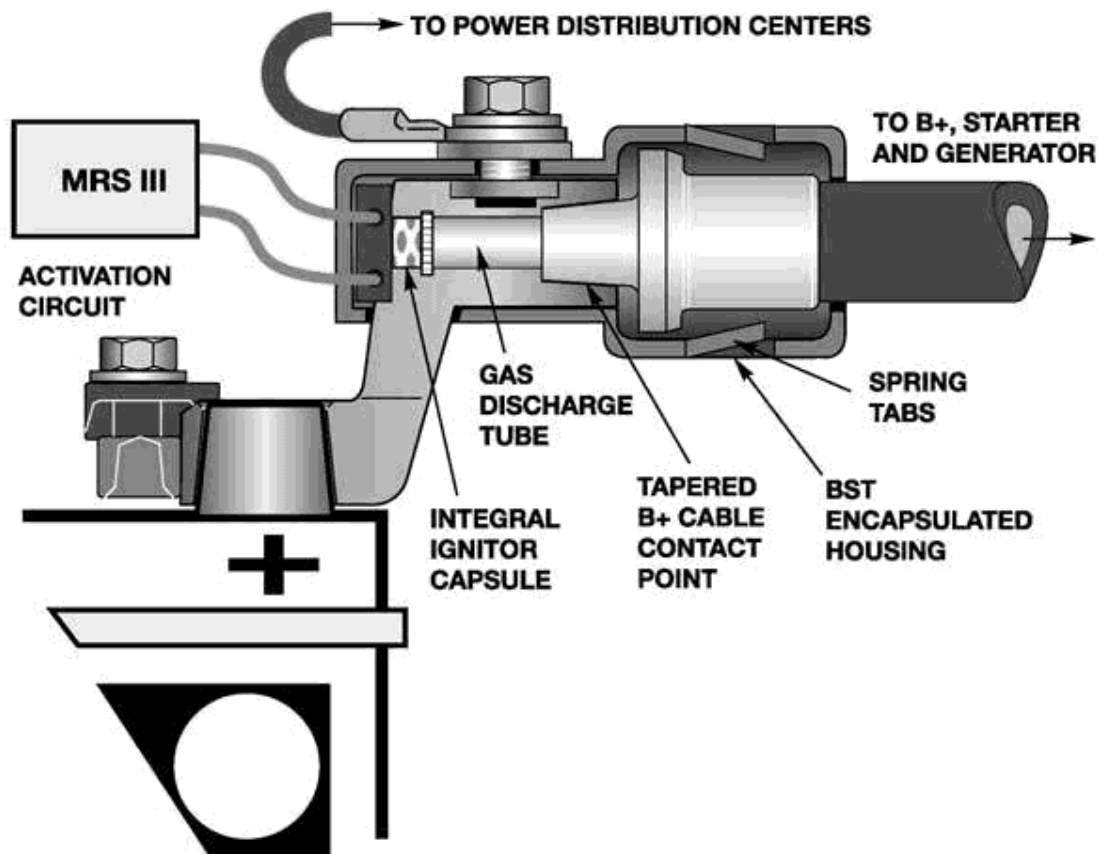
Fig. 10: Identifying Battery Safety Terminal (BST) Courtesy of BMW OF NORTH AMERICA, INC.
