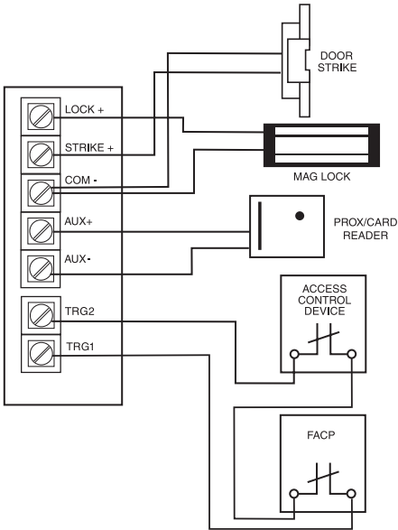
Fig. 4 - Typical mag lock with fire alarm tie-in using aux output installation:
