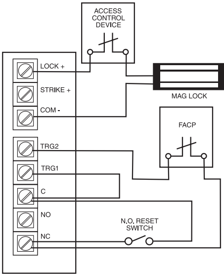
Fig. 5 - Latching fire alarm tie-in with manual reset:
