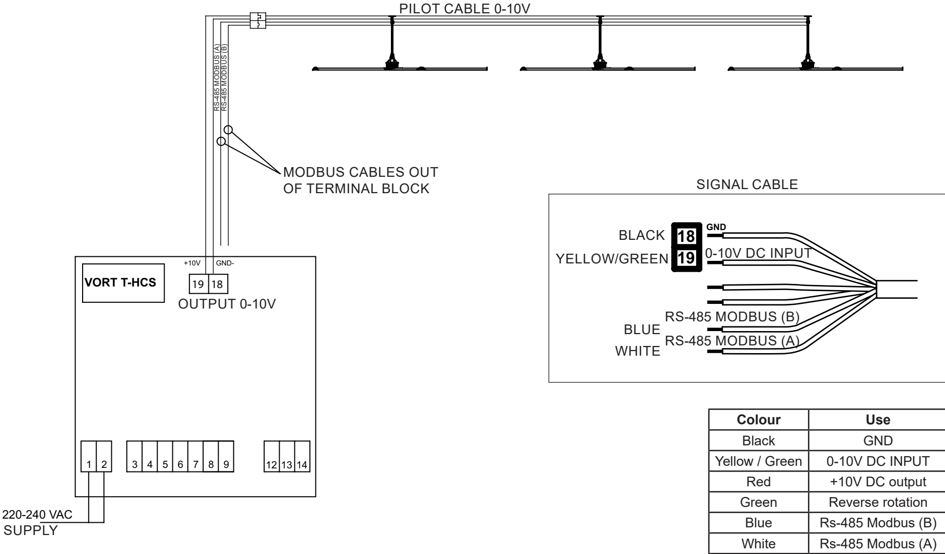
CONNECTION DIAGRAM WITH “VORT T-HCS” CONTROL UNIT (CODE 20.151)
