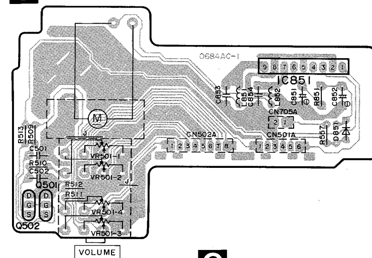
G OPERATION P.C.B.
