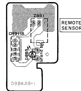
I REMOTE SENSOR P.C.B.
