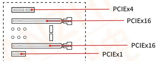
2-4 PCI Expansion Slot
