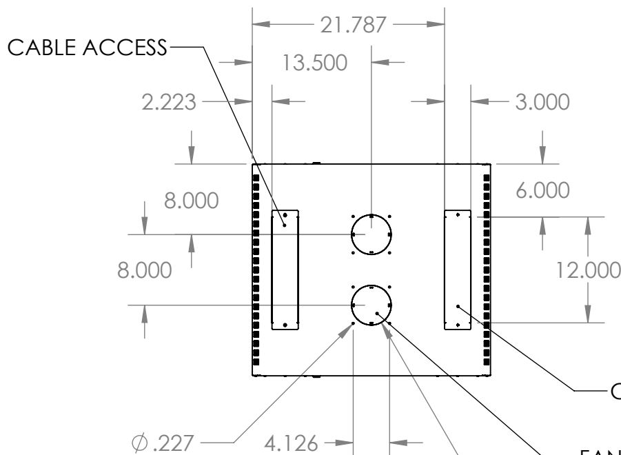
VIEW B-B SCALE 1 : 15 TOP VIEW
