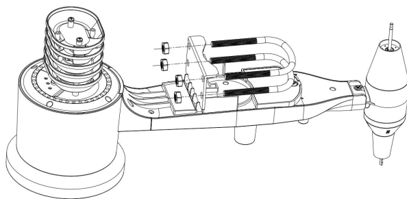
Figure 3: U-Bolt installation
