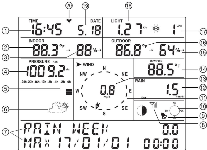
Figure 10: Display Console Screen Layout
