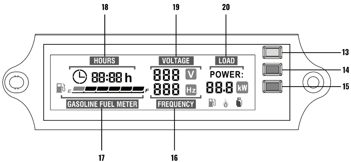
Diagram 3. Display Function
