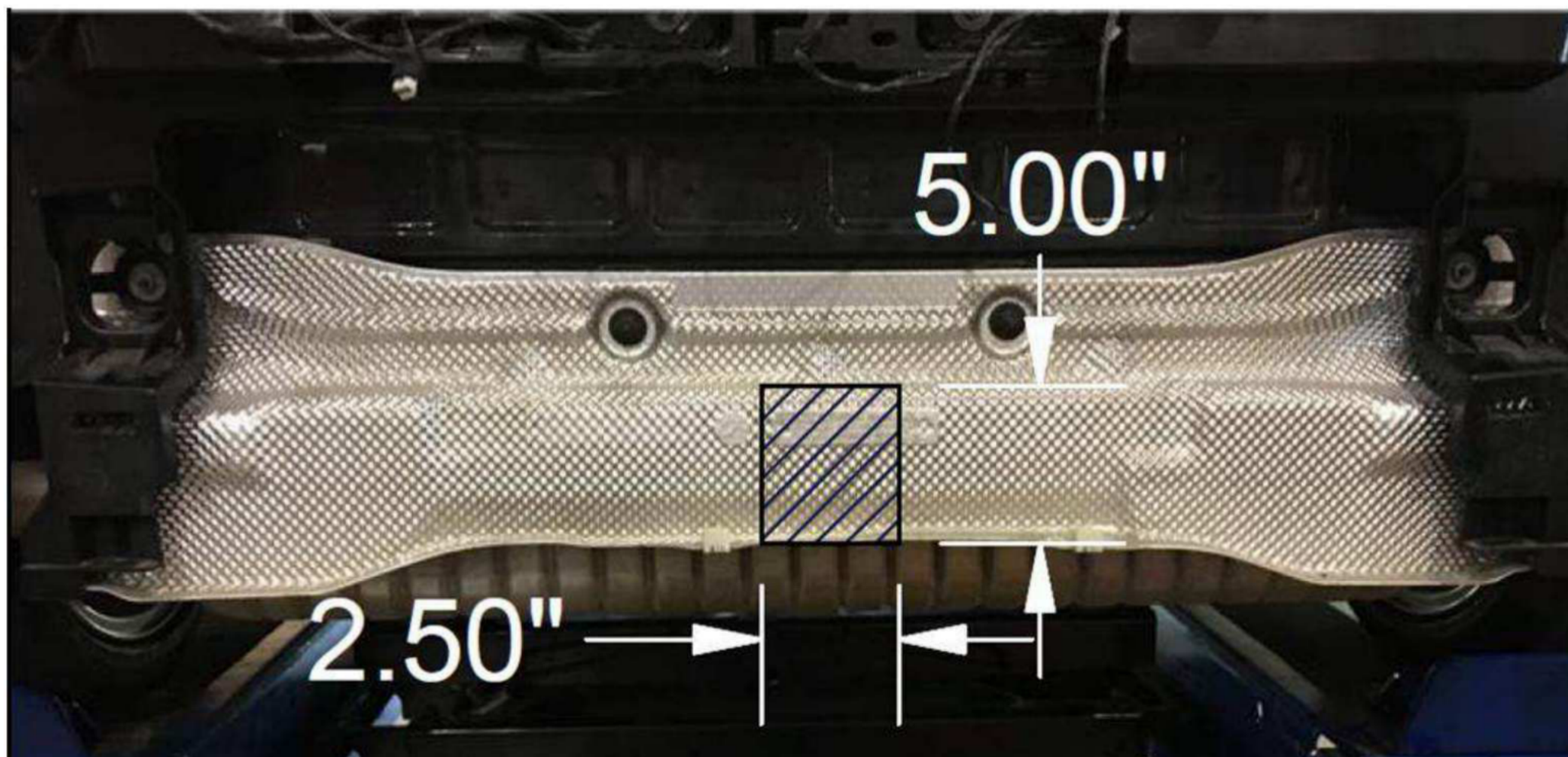
TRIM DIAGRAM
