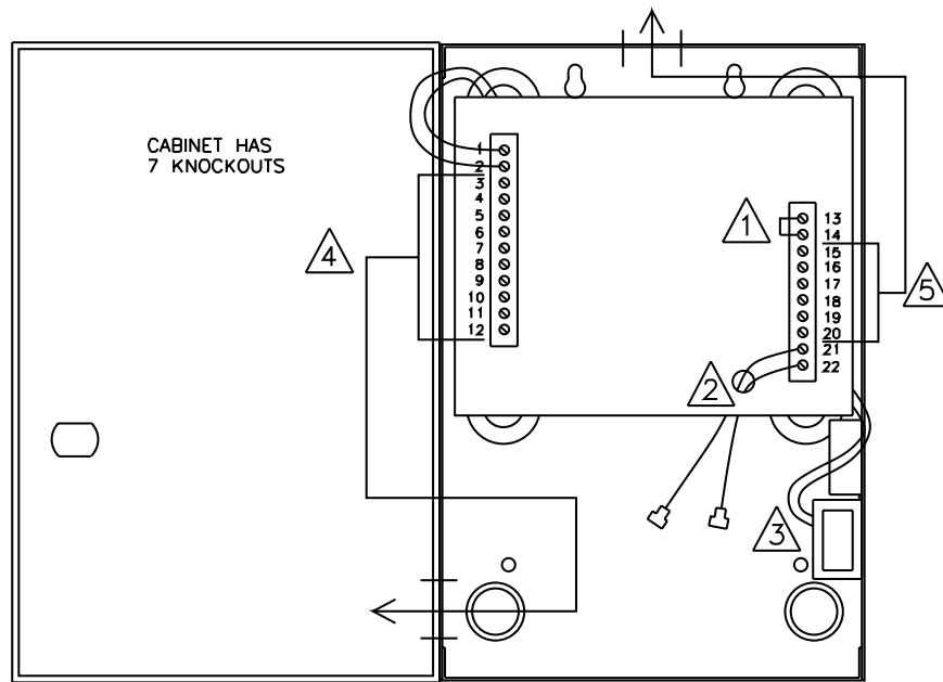
FIG. 4 WIRE ROUTING
