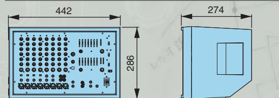
Rear Panel
