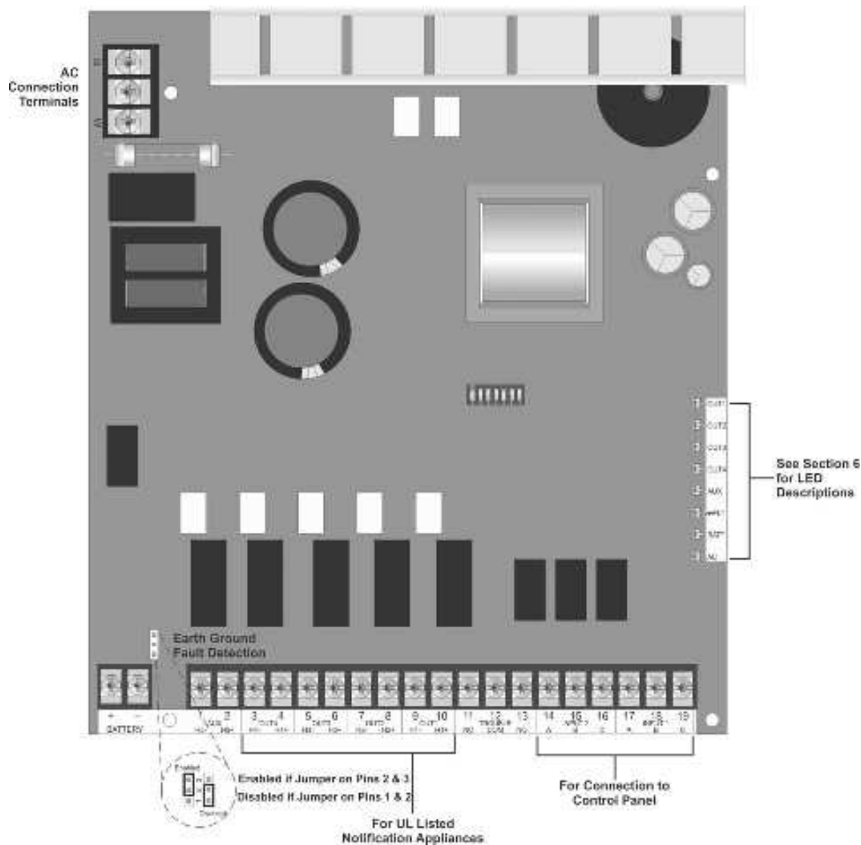
Figure 4-2 The Model HPF902ULADA PC Board Layout
