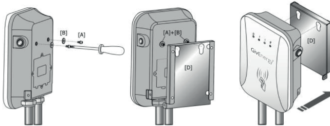
Fig. 1.7 Mounting the charging station
