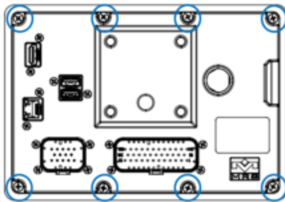
Figure 2: Schematic representation – Back of the MConn 7 and localisation of the eight Phillips screws (blue circles).
