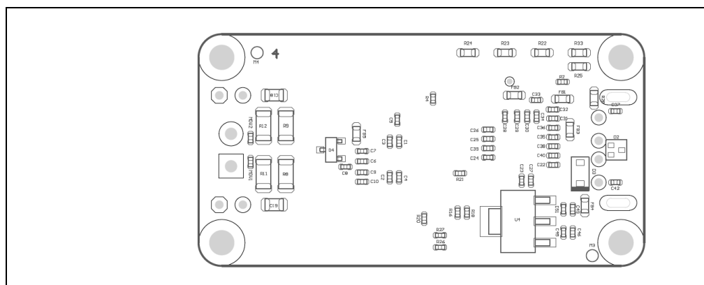
FIGURE 3-2: ASSEMBLY PLAN – BOTTOM VIEW
