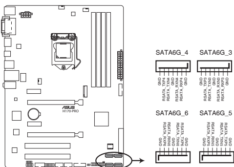
H170-PRO Intel® SATA 6.0Gb/s connectors
