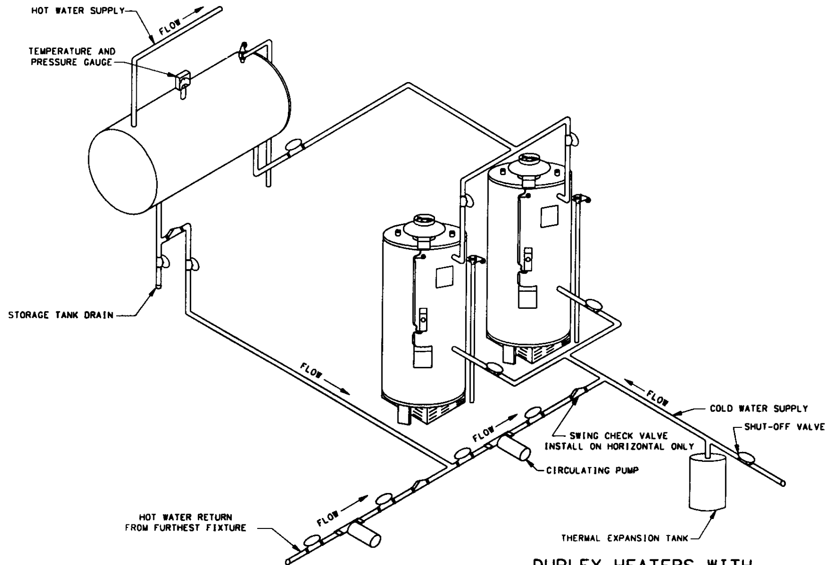
DUPLEX HEATERS WITH HORIZONTAL STORAGE TANKS SEE NOTES ON PAGE TWO PRIOR TO INSTALLATION
