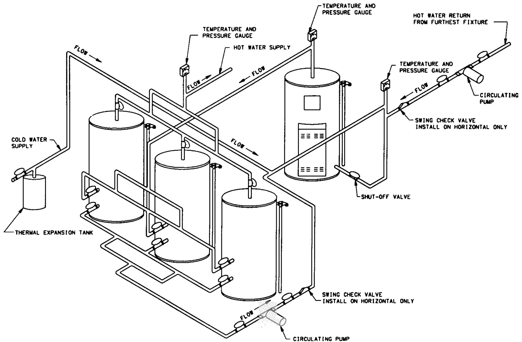
SINGLE HEATER WITH TRIPLEX STORAGE TANKS SEE NOTES ON PAGE TWO PRIOR TO INSTALLATION
