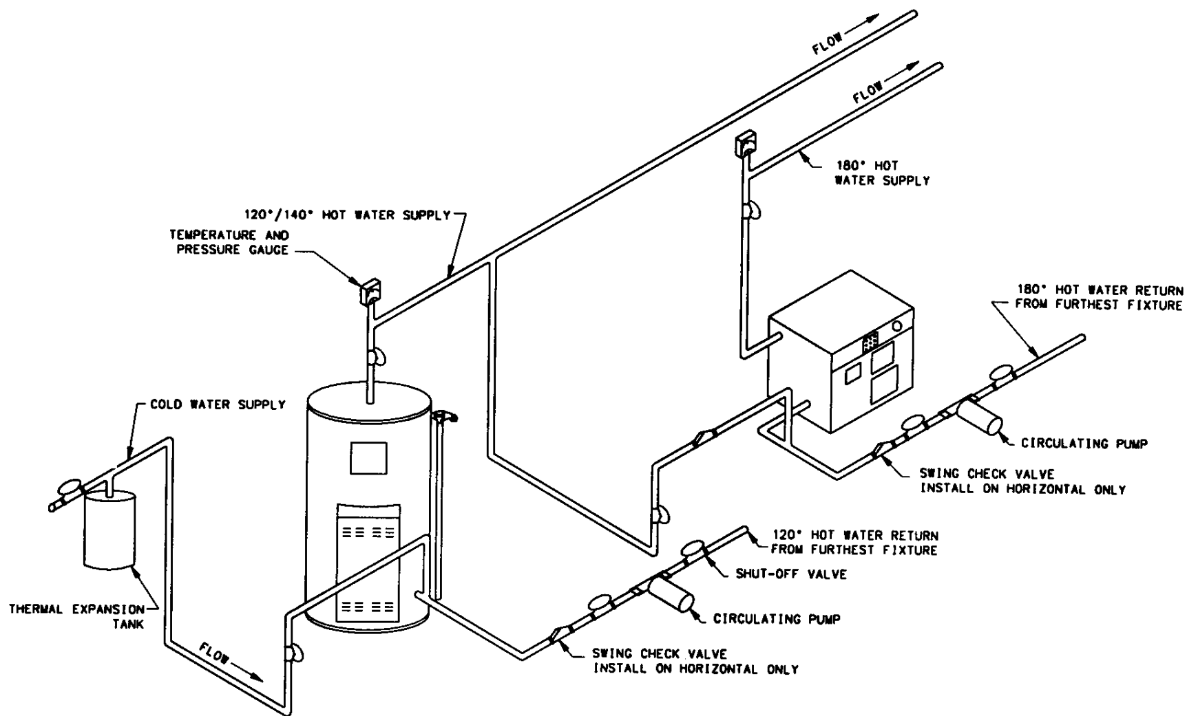
DUAL TEMPERATURE WITH BOOSTER HEATER
