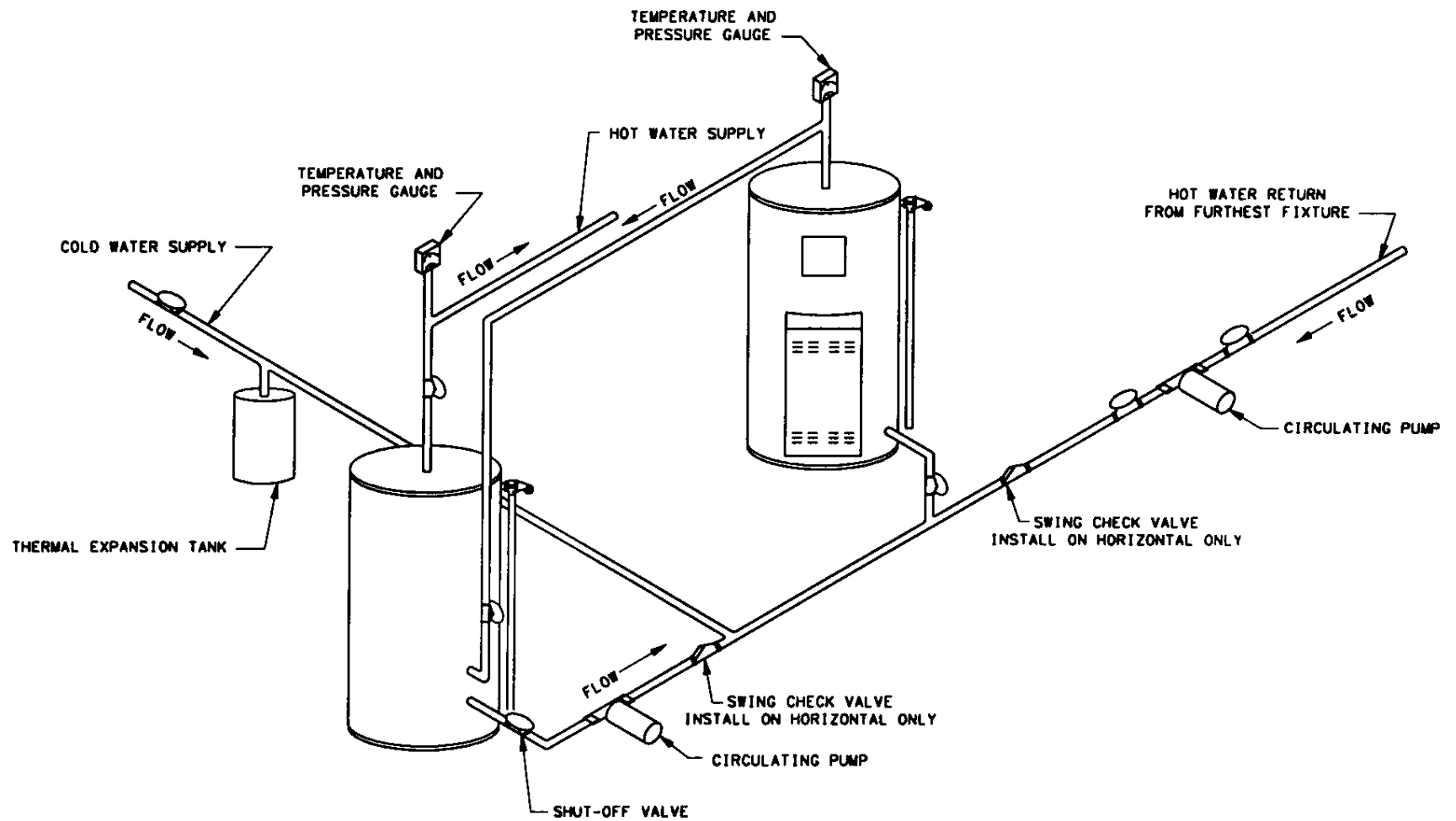
SINGLE HEATER WITH STORAGE TANK SEE NOTES ON PAGE TWO PRIOR TO INSTALLATION
