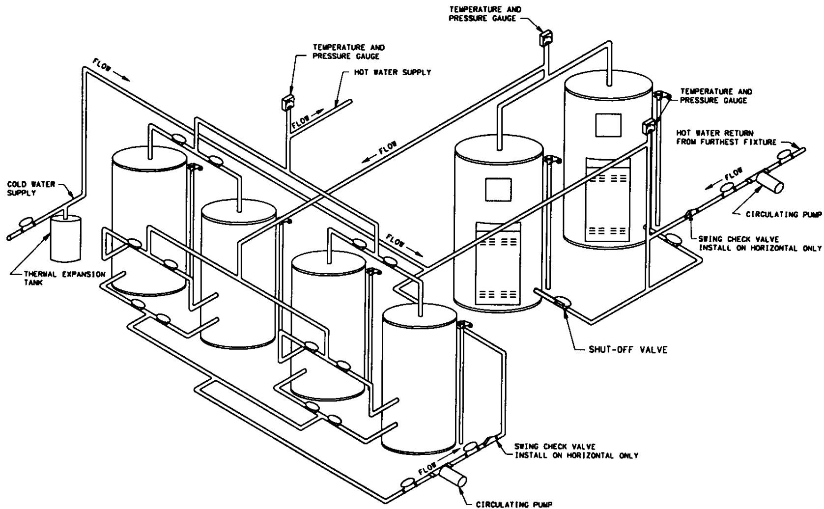
DUPLEX WITH QUADPLEX STORAGE TANKS SEE NOTES ON PAGE TWO PRIOR TO INSTALLATION
