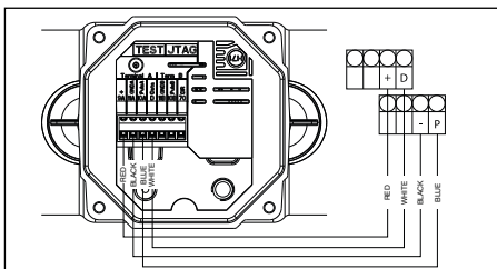
Connection AXONIC/CF800
