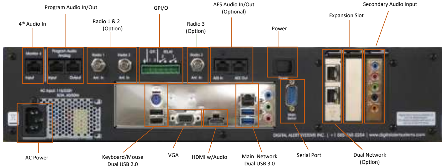
Back Panel View of the DAS3-GX or DAS3-EX with DAS3-AES and EXP-2NICGIG options
