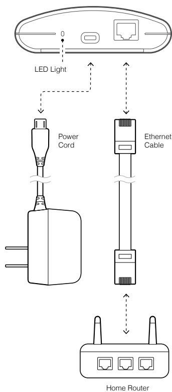
GATEWAY ULTRA Module (side view)
