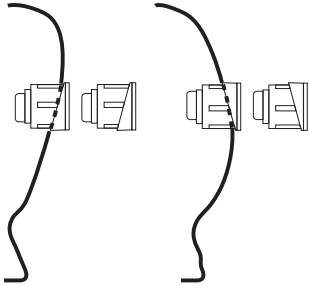
Installation when bumper is sloping to the ground.
