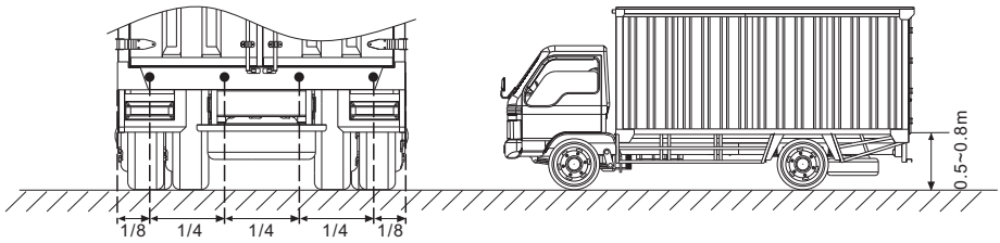
Best position for 4 sensors
