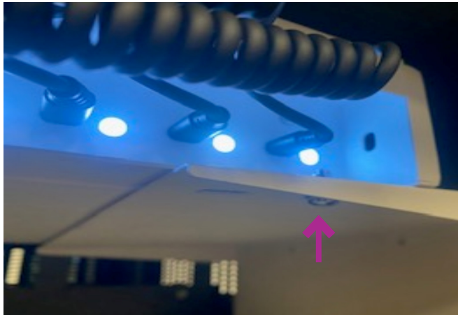
Spring Washer
