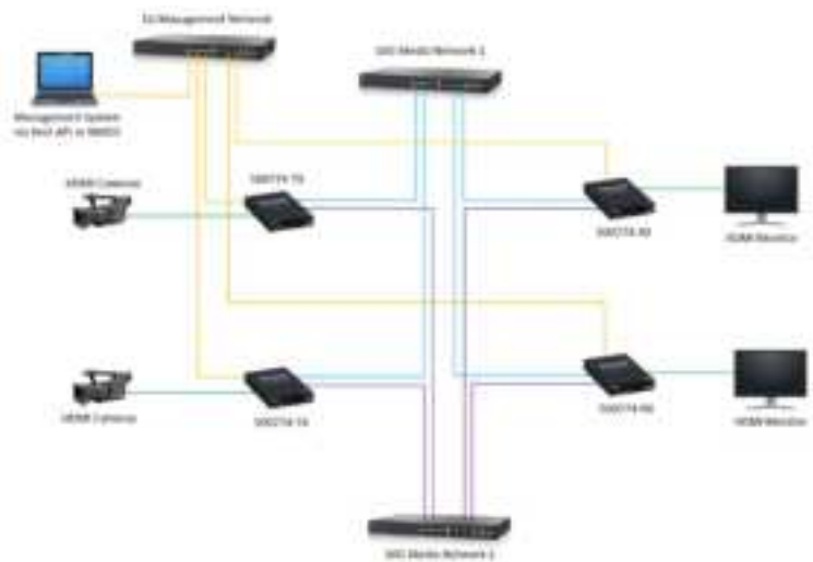
Figure 2b: Application Diagram with redundancy (without Fault)
