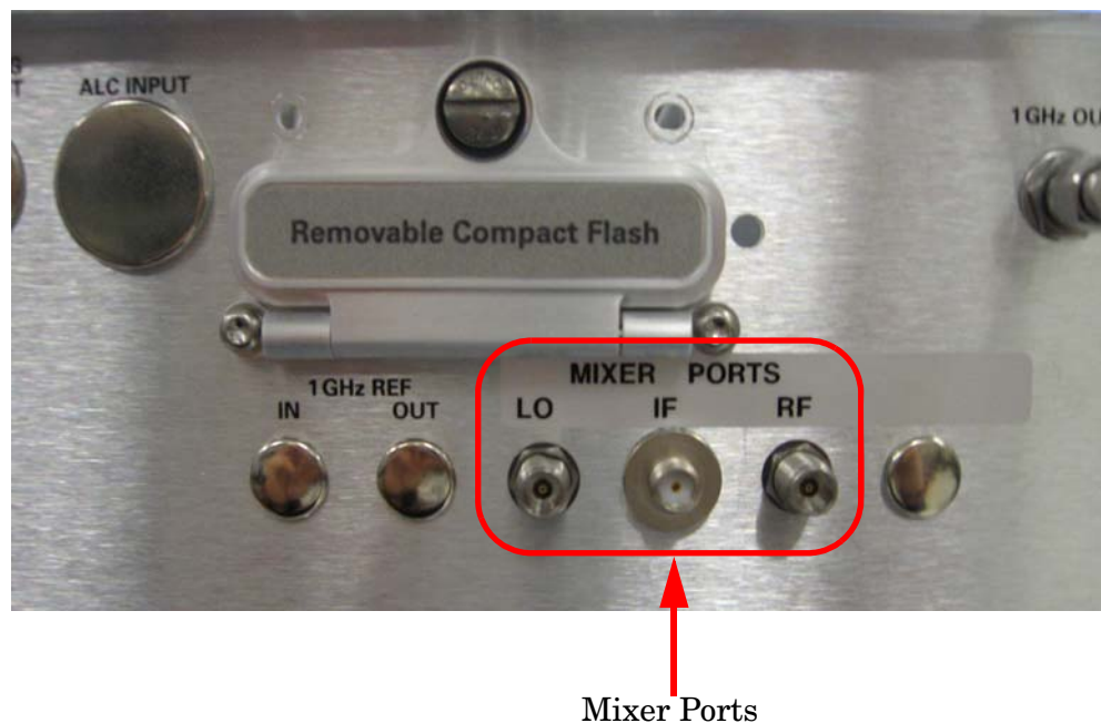
Figure 3 Rear Panel
