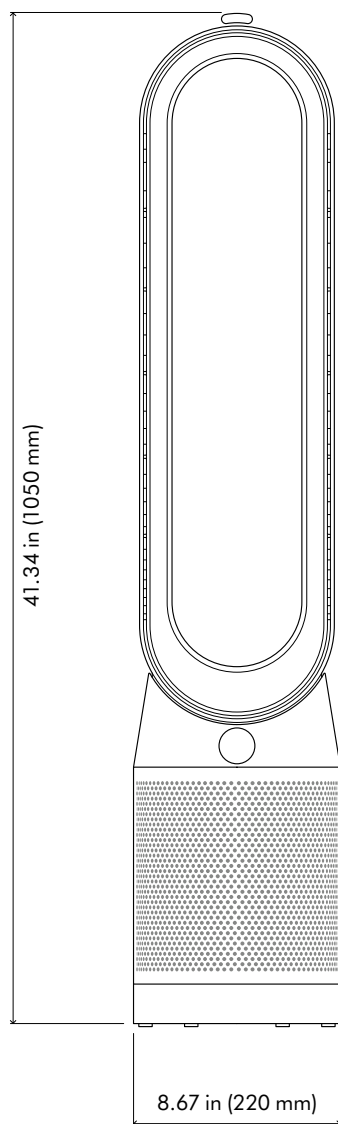
Front elevation
