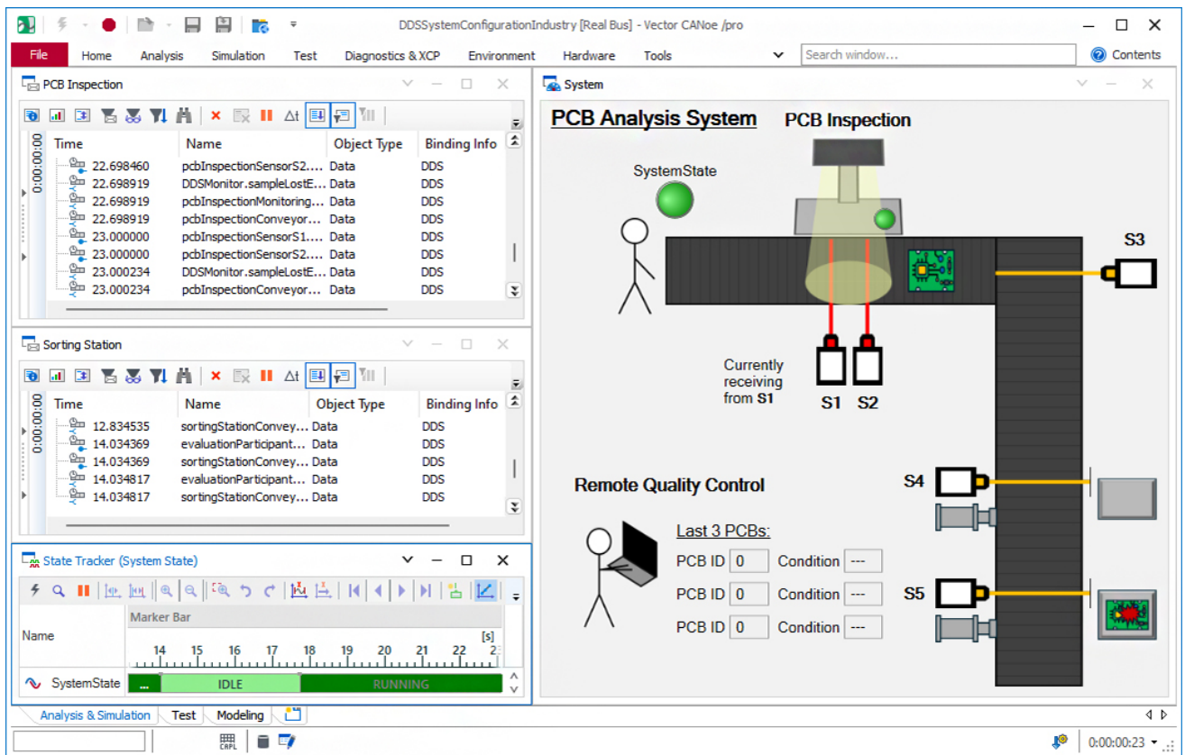
Figure 2: An example of a simulation and visualization of a DDS system in CANoe
