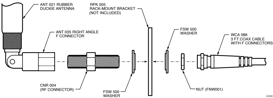
Figure 1: ANT 034 Assembly
