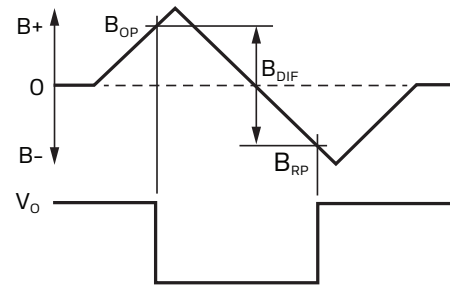
FIGURE 4. TRANSFER CHARACTERISTICS DEFINITION
