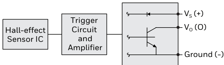
FIGURE 5. CURRENT SINKING OUTPUT BLOCK DIAGRAM
