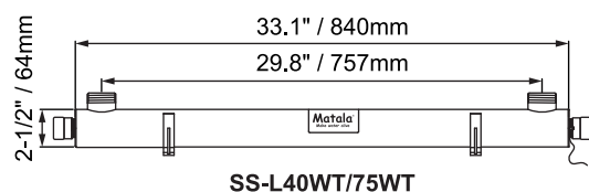
SS-L40WT/75WT
