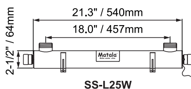
SS-L25W
