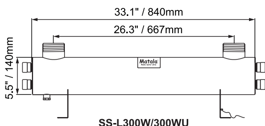
SS-L300W/300WU
