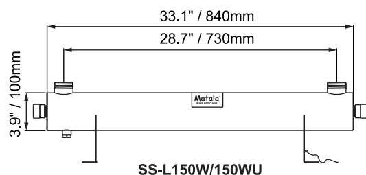
SS-L150W/150WU
