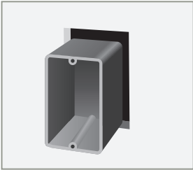
When installing jamb version, cutout dimensions are 1 1/2" (W) x 2 7/8" (H) x 1" (D min)
