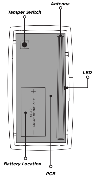
Figure 2: PCB Components
