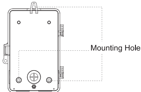
FIG.4 Mounting Holes
