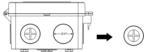
FIG.3 3/4" knockout
