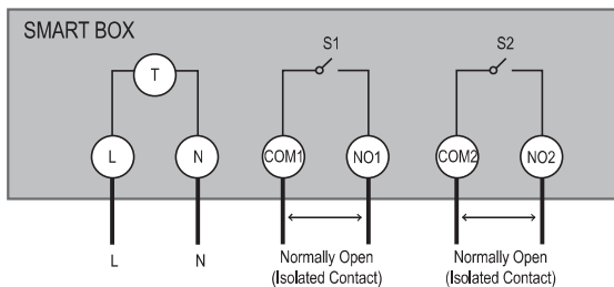
FIG.5 TERMINAL DESIGNATIONS
