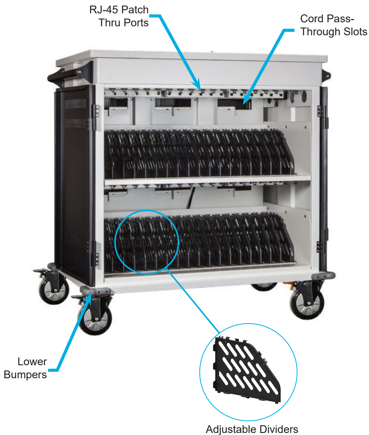
Front View of Cart
