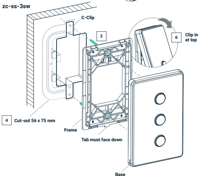
zc-ss-3sw
