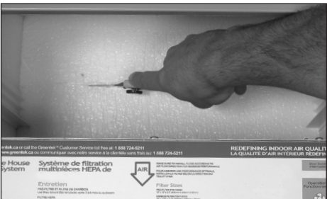
Figure 2.2b - One cut permits the clean removal of the insulation piece.
