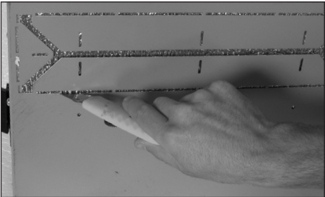
Figure 2.2a - Cut insulation along the inside edge of both of the inlet and outlet ports to remove the insulation from the port openings.
