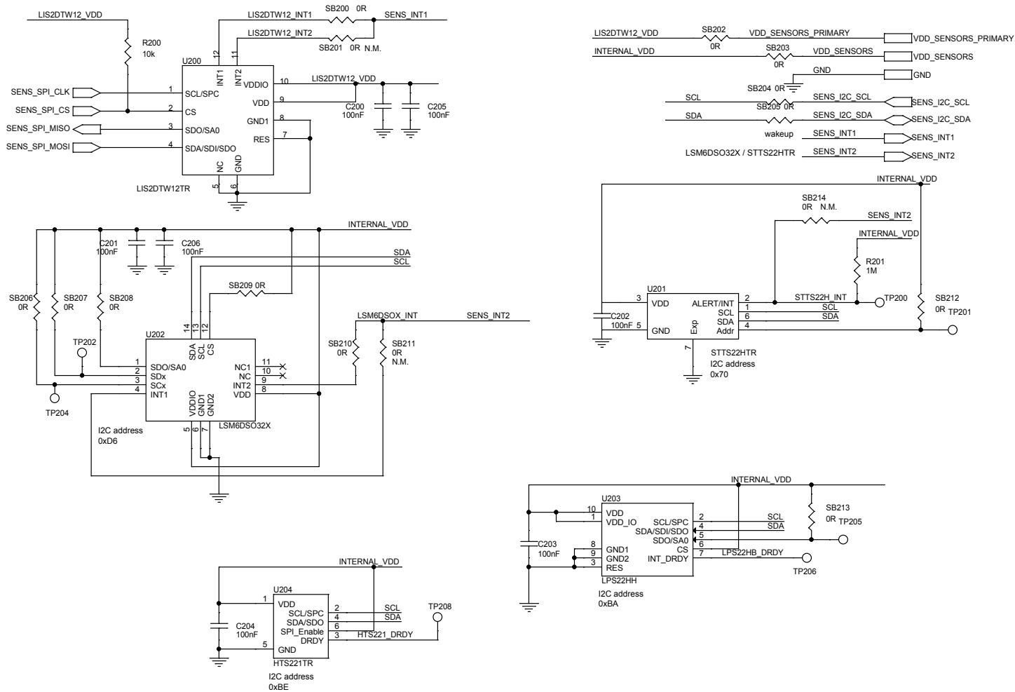
Figure 49. Main board (STEVAL-ASTRA1) circuit schematic (8 of 9)
