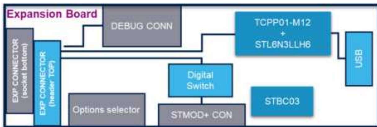
Figure 23. Expansion board block diagram
