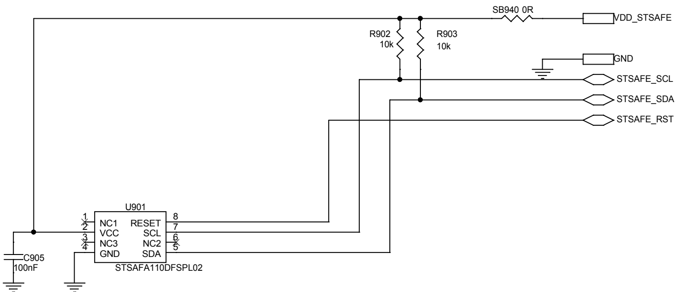
Figure 57. System on board (STEVAL-ASTRA1SB) circuit schematic (7 of 10)
