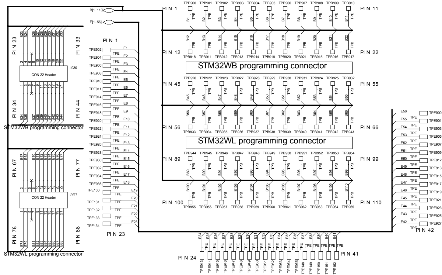
Figure 54. System on board (STEVAL-ASTRA1SB) circuit schematic (4 of 10)
