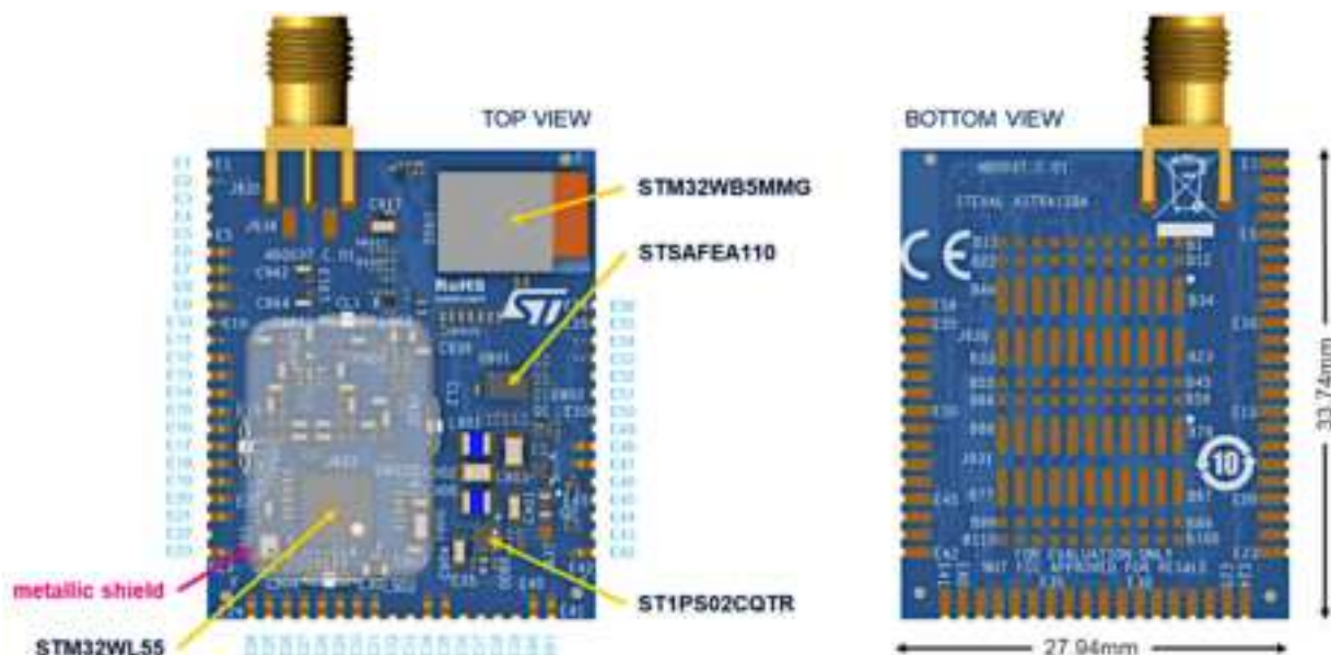
Figure 4. System on board - main component placement and pinout
