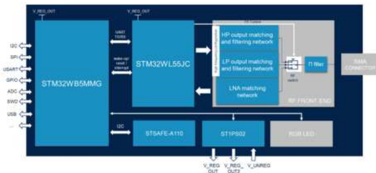
Figure 3. Block diagram of the STEVAL-ASTRA1SB system on board
