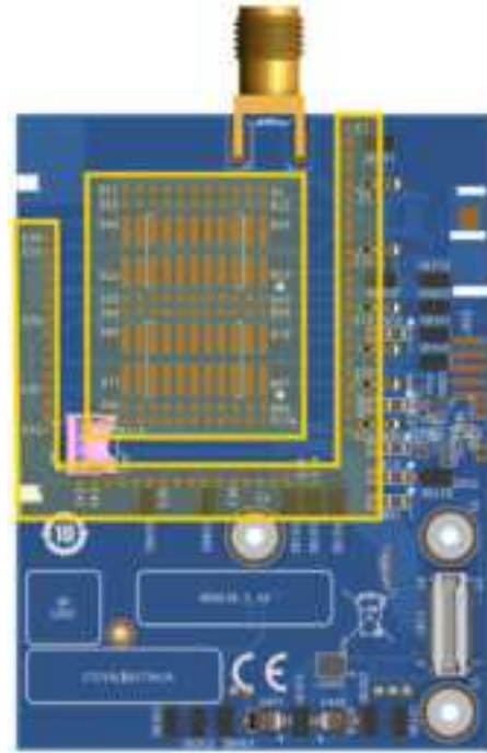
Figure 19. Bottom pads
