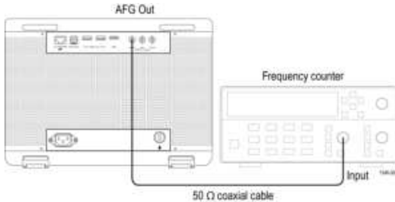
Figure 1: Frequency/period test
