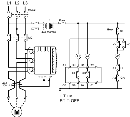
Three phase motor (D type, b-a output)
