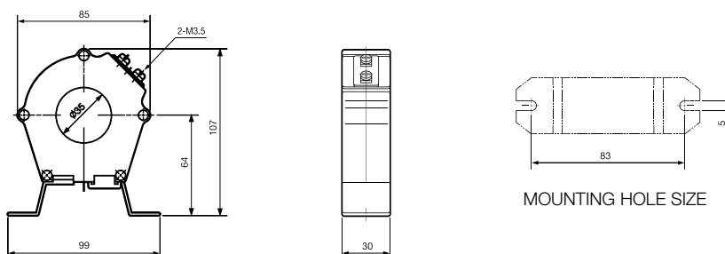
ZCT-Ø35
