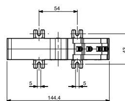
MOUNTING HOLE SIZE
