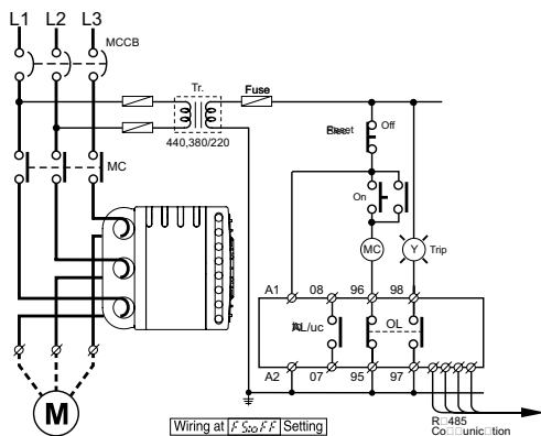
Typical wiring for EOCR-i3DM / iFDM ( 3 phase motor - window type)
