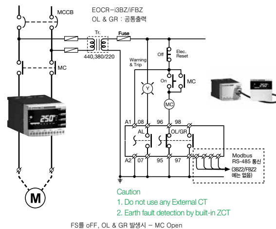
Single phase line Diagram
