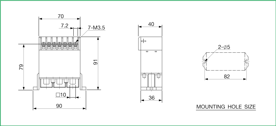
EOCR-DG (Hole Type)
