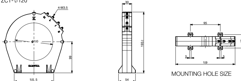
ZCT-Ø120
