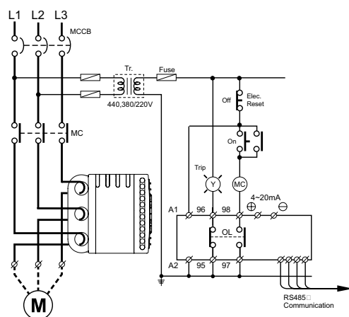
Typical wiring for EOCR-i3M420 / iFM420
