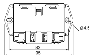
MOUNTING HOLE SIZE
