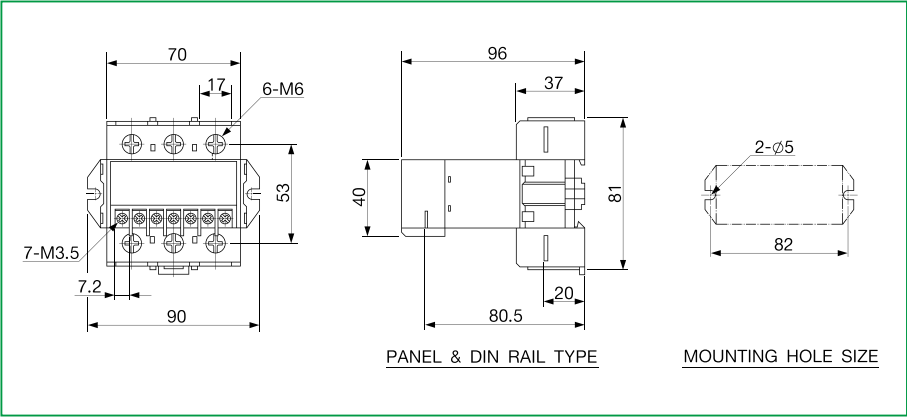
EOCR-DGT (Terminal Type)
