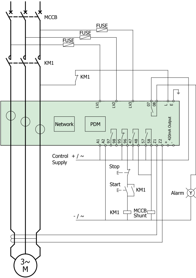
Direct On Line (DOL) Starter
