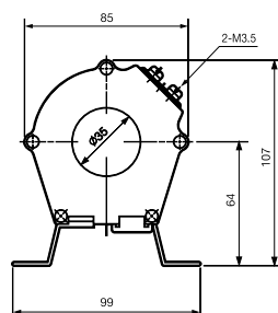
ZCT-Ø35
