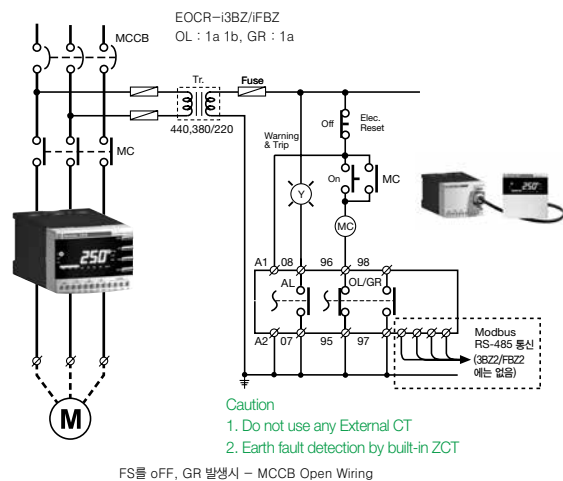
3 phase line Diagram
