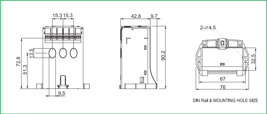
EOCR-SE2
