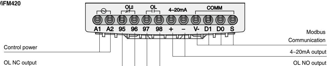
EOCR-i3M420/iFM420
