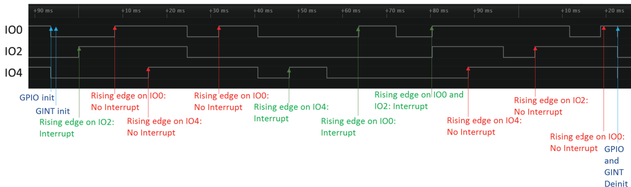
Fig 40. GINT Example for “(IO0 asserted) OR (IO2 asserted) OR (IO4 asserted)”
