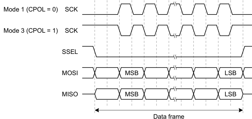
Fig 61. Basic SPI operating modes
