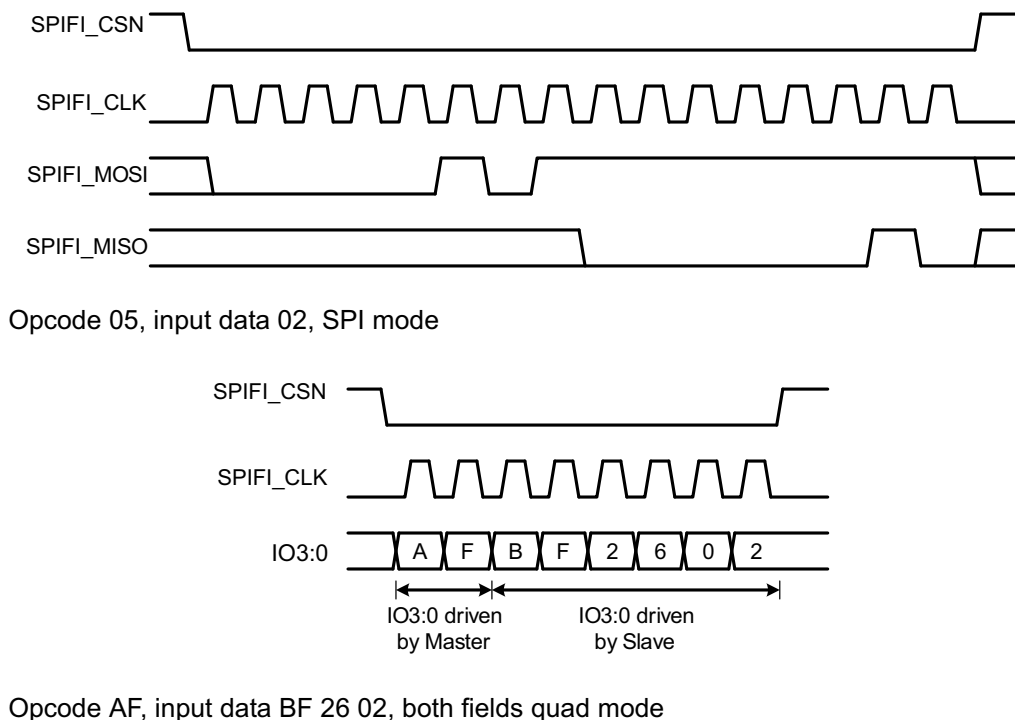
Fig 87. Read commands
