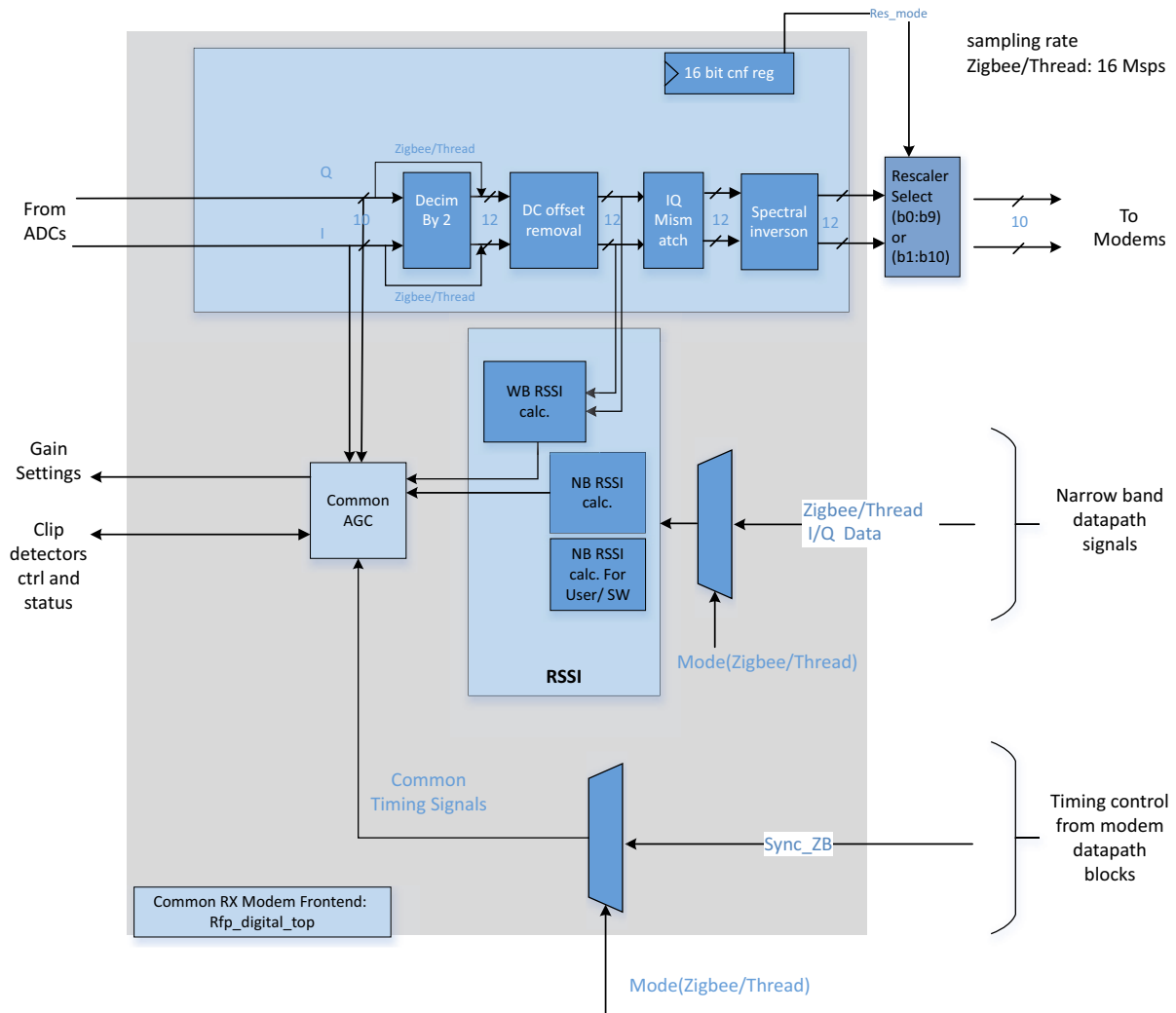
Fig 114. RFP RX Datapath architecture
