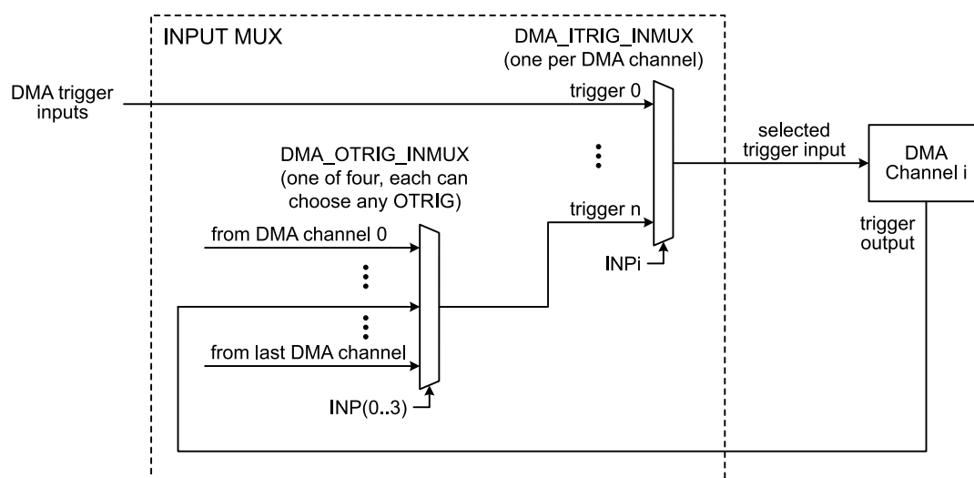
Fig 32. DMA trigger multiplexing
