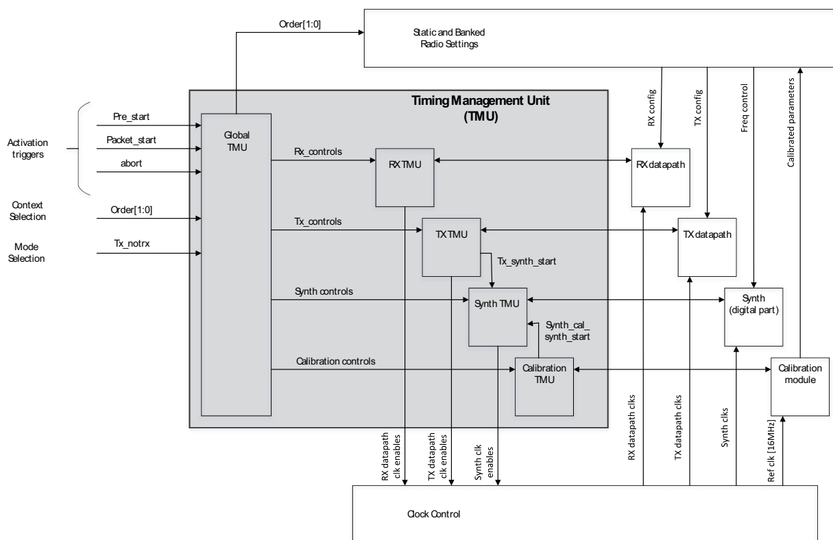
Fig 110. TMU architecture
