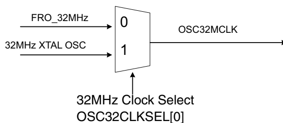
Fig 8. 32 MHz clock sources internal muxing
