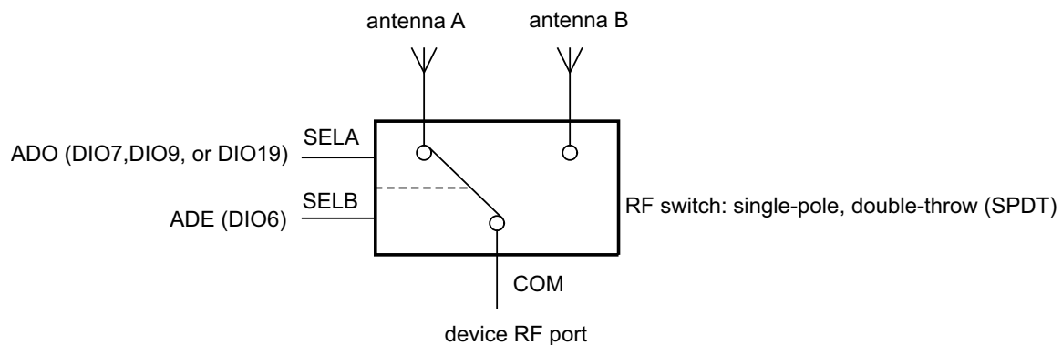
Fig 122. Simple antenna diversity implementation using external RF switch
