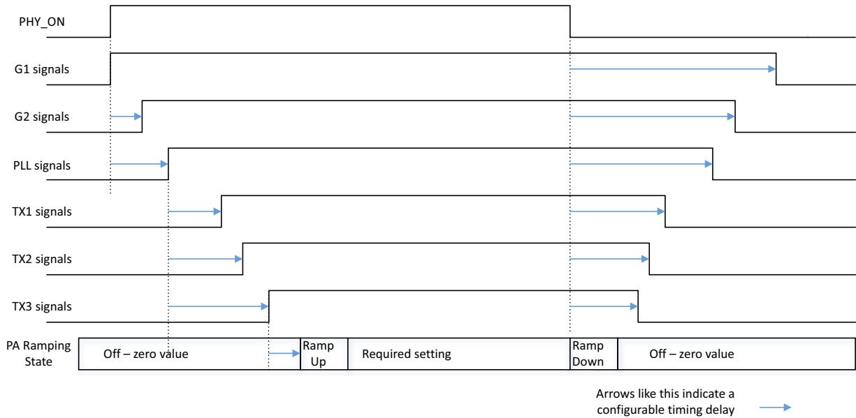
Fig 112. Transmit sequence of group enables
