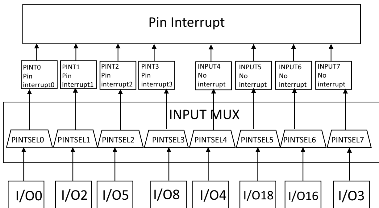
Fig 34. Pattern Match Engine
