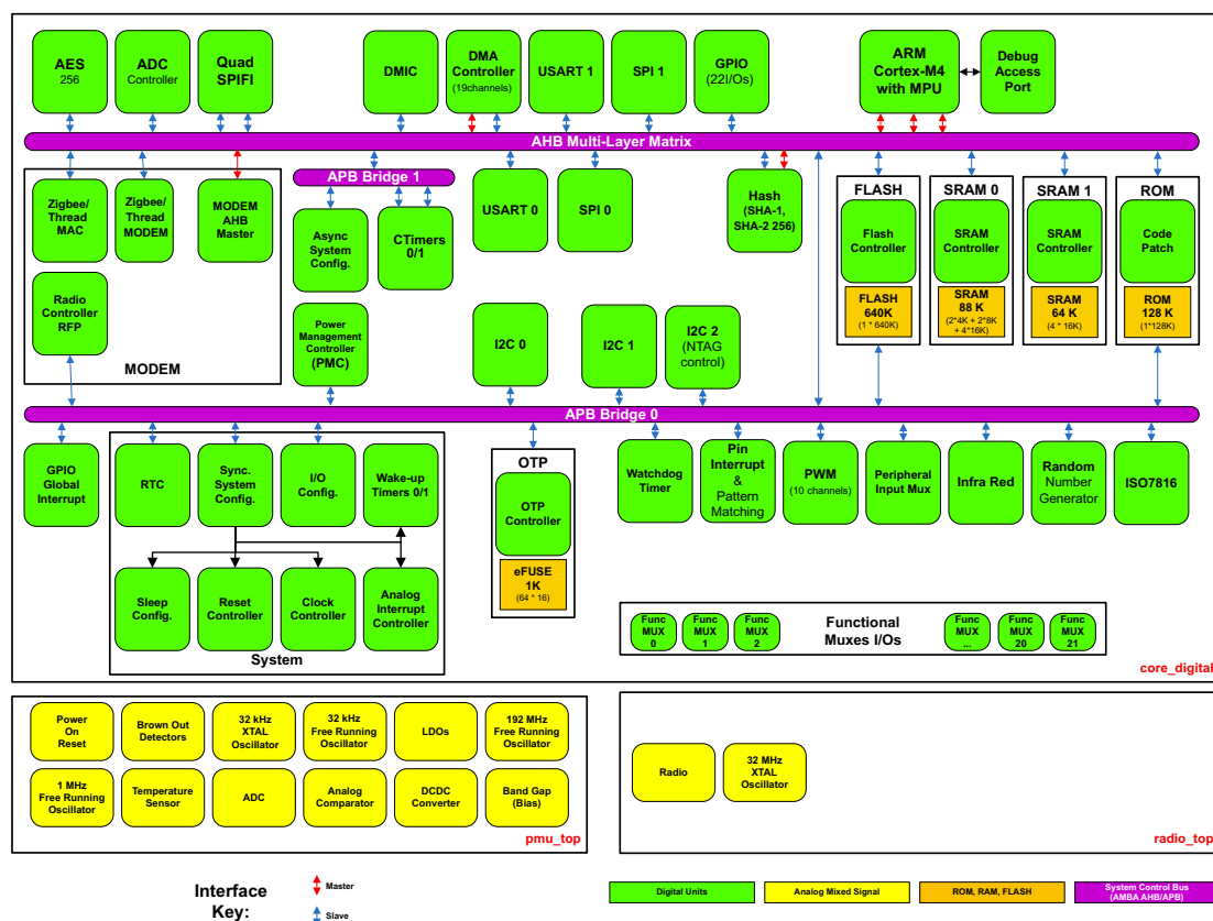
Fig 1. Chip block diagram
