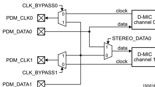
Fig 67. DMIC subsystem pin multiplexing
