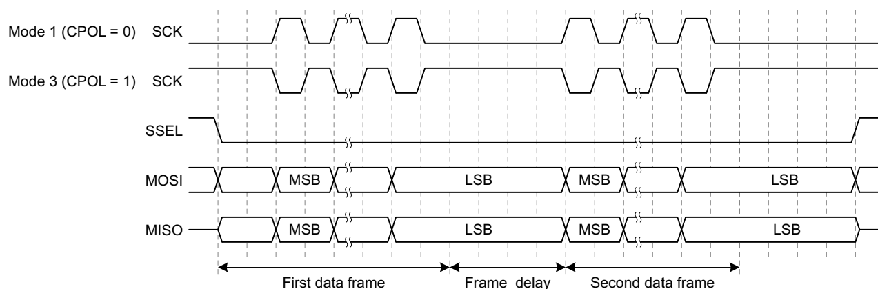
Fig 63. Frame_delay
