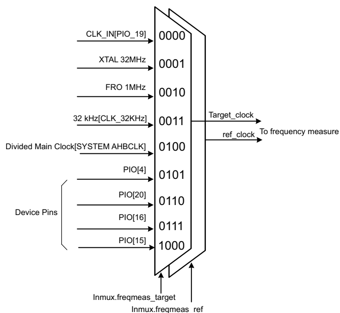
Fig 98. Clock sources to frequency measure block diagram
