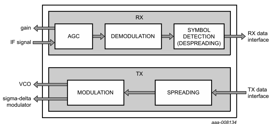
Fig 118. Modem architecture
