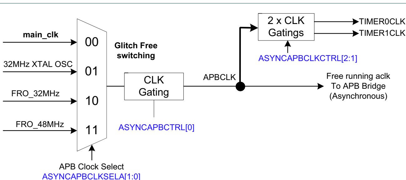
Fig 10. APB clock generation
