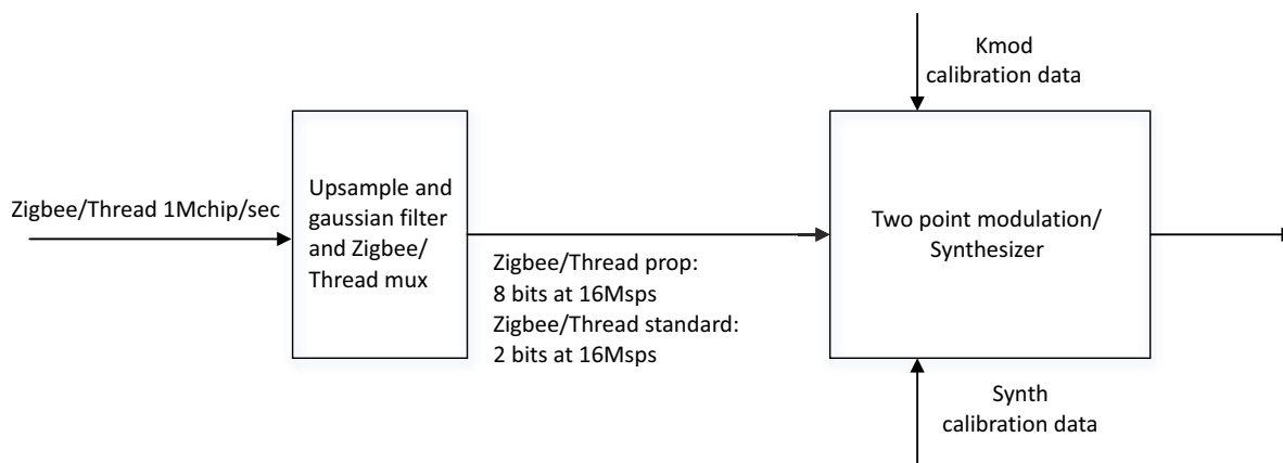
Fig 113. Transmit datapath architecture
