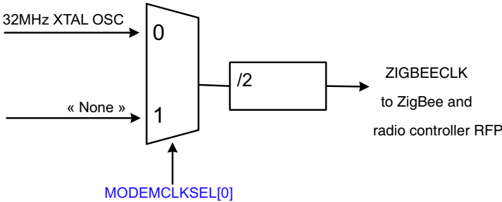
Fig 16. Zigbee/Thread clock selection
