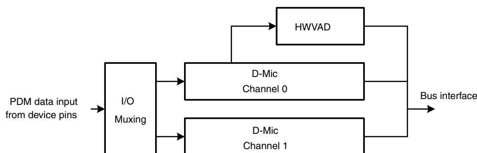
Fig 72. DMIC subsystem block diagram
