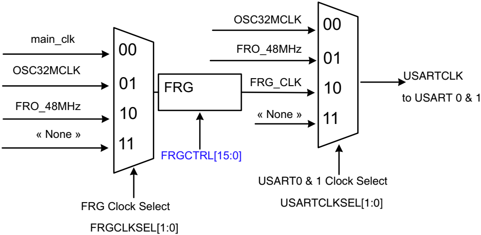
Fig 14. USART clocks selection
