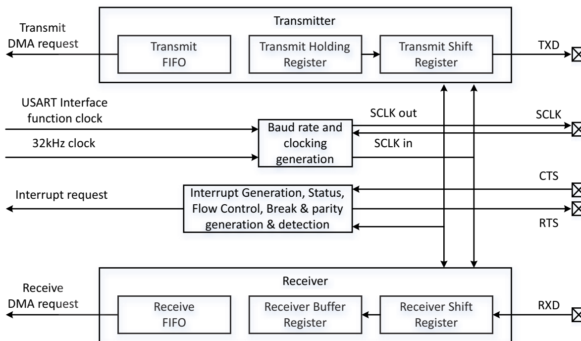
Fig 58. USART block diagram
