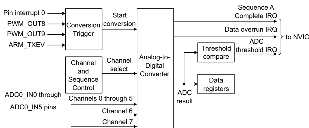
Fig 82. ADC block diagram
