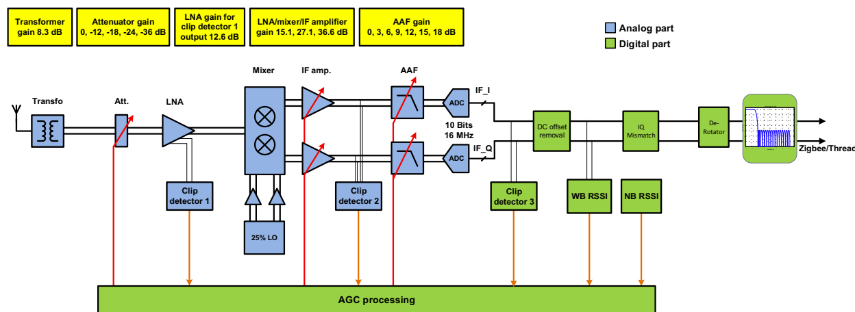
Fig 115. Receiver simplified block diagram for AGC
