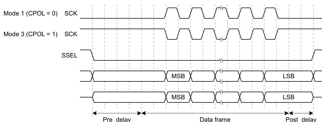
Fig 62. Pre_delay and Post_delay
