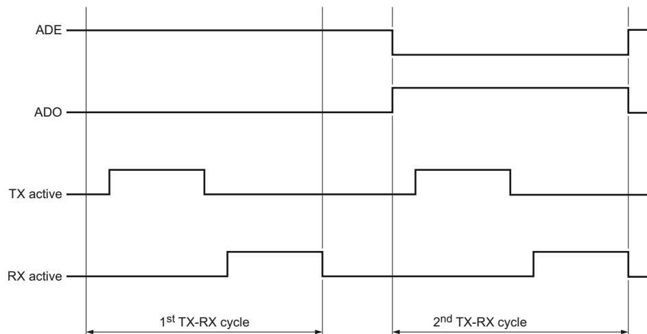
Fig 123. Zigbee/Thread antenna diversity ADO and ADE signals for TX with acknowledgment
