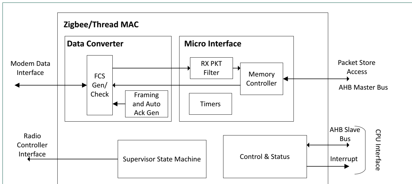
Fig 121. Zigbee/Thread MAC block diagram
