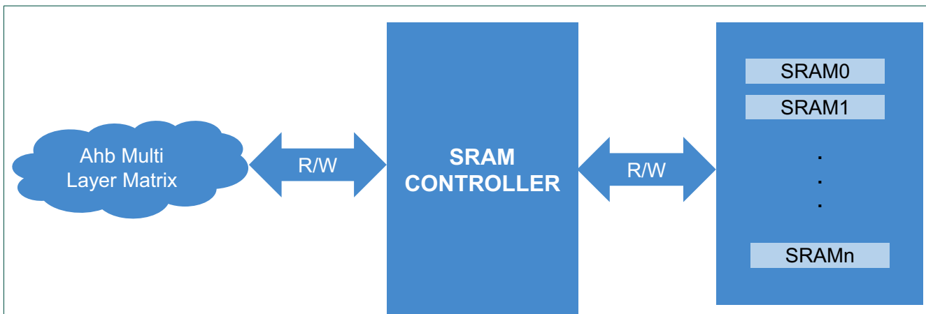
Fig 84. SRAM controller connection
