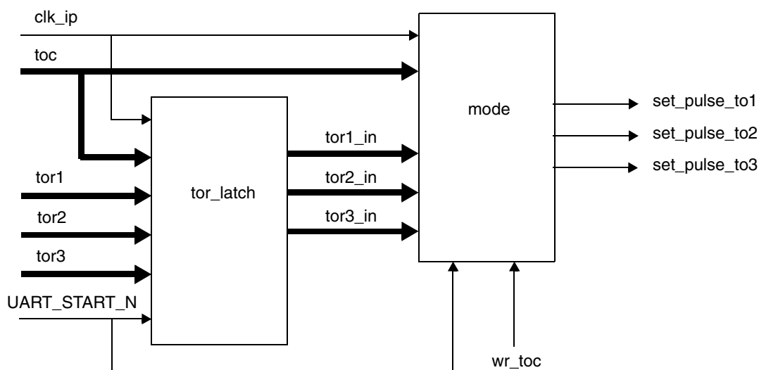
Fig 93. Timer block diagram
