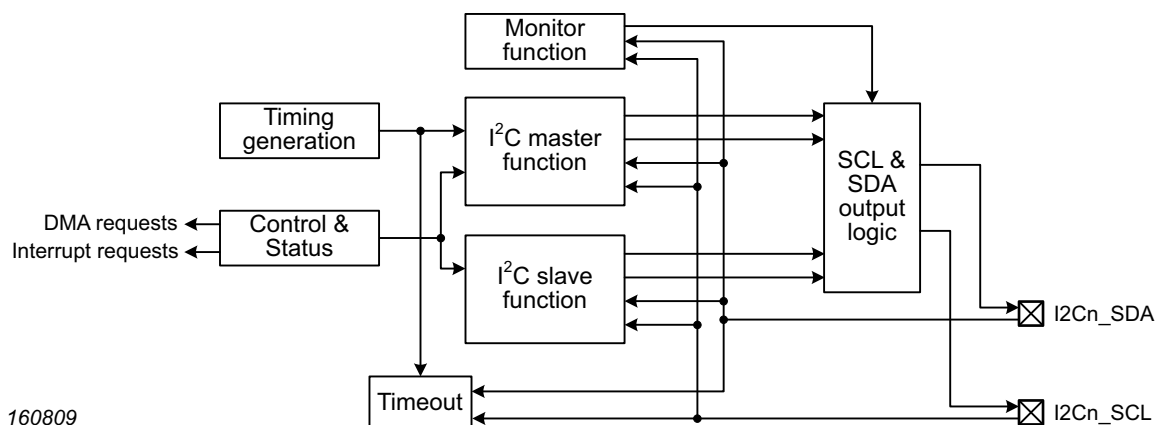
Fig 66. I 2 C block diagram
