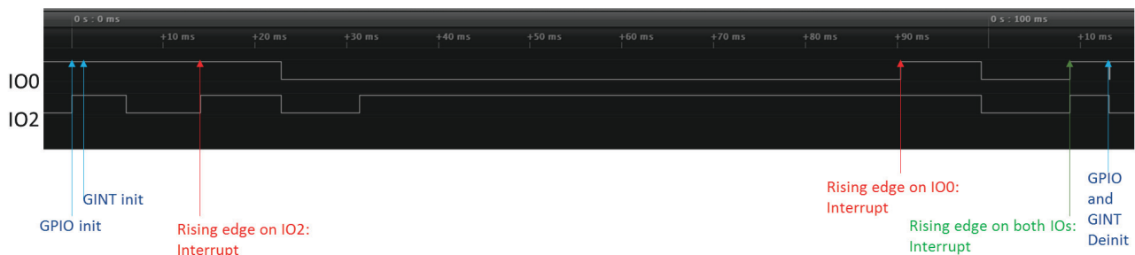
Fig 41. GINT example for “(IO0 asserted) AND (IO2 asserted)”
