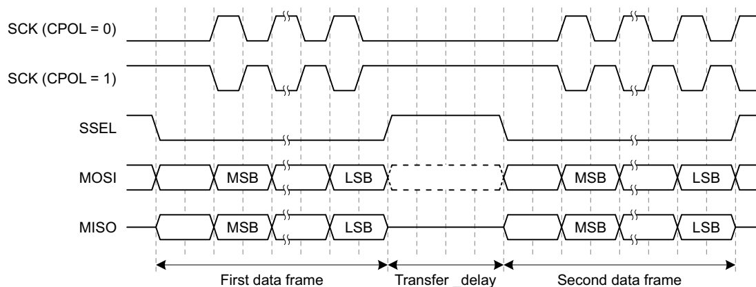
Fig 64. Transfer_delay
