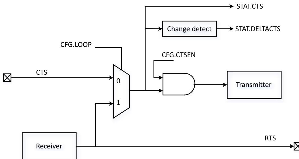
Fig 59. Hardware flow control using RTS and CTS
