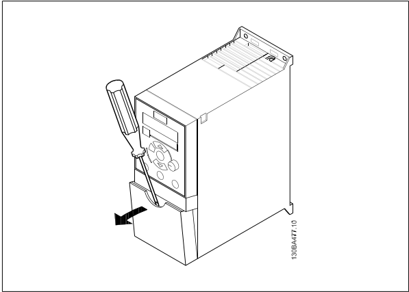
3.6: Removing the terminal cover.
