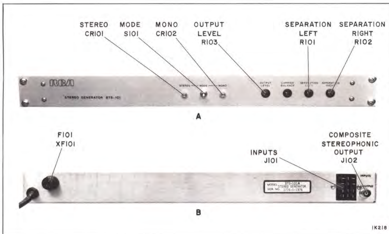
Figure 1. BTS-101A External Views
