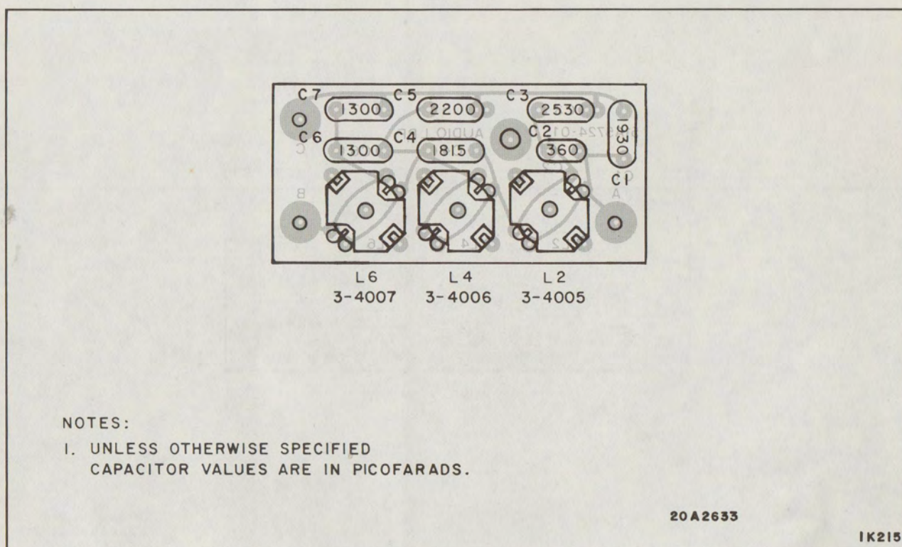
Figure 9. Audio Lowpass Filter Components Location
