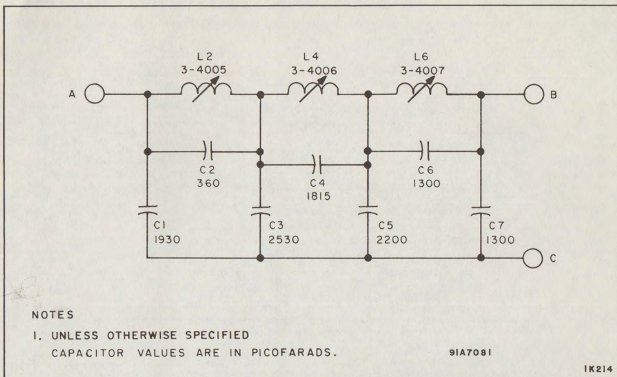
Figure 8. Audio Lowpass Filter Schematic
