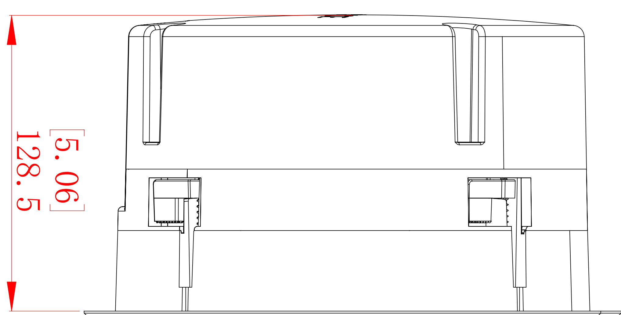
MOUNTING DEPTH
