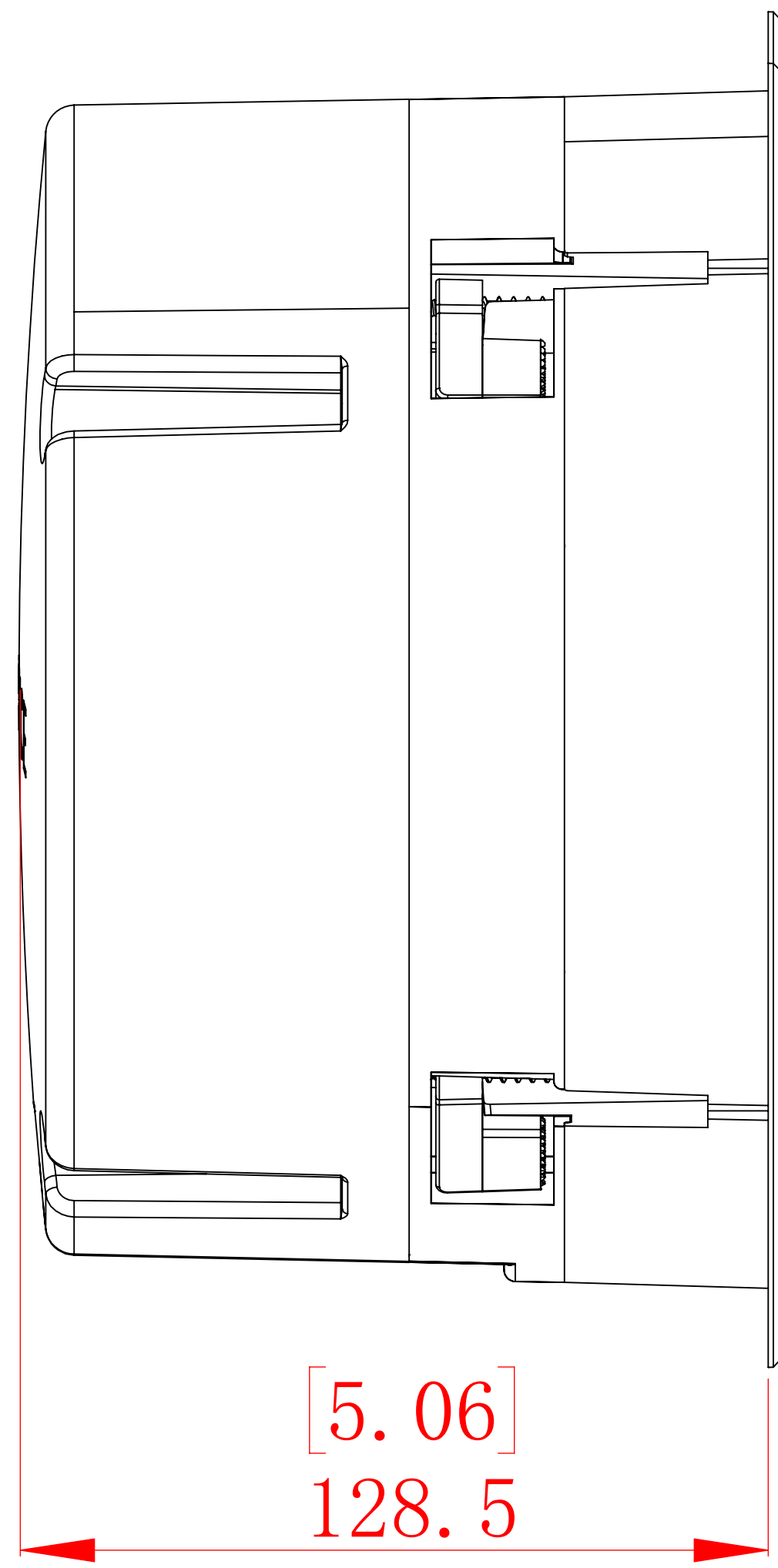
MOUNTING DEPTH
