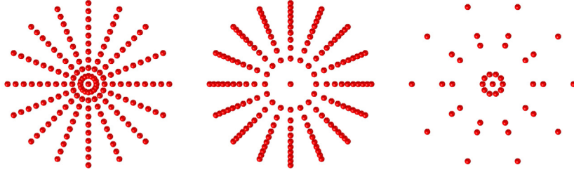
Figure 3-6: Comparison of the cylindrical release in which rays are positioned at uniform radius intervals (left), with uniform number density (center), or at user-defined radii (right).
