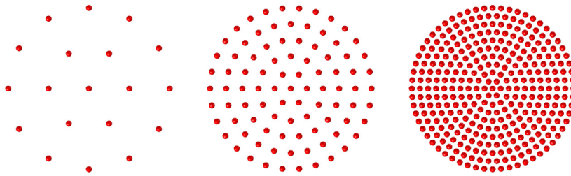
Figure 3-7: Comparison of hexapolar grids with 2 rings (left), 5 rings (middle), and 10 rings (right).
