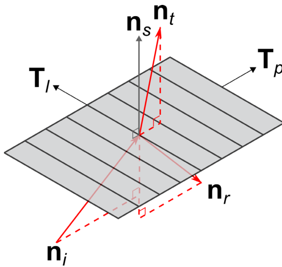
Figure 3-5: Diagram illustrating the options to specify grating orientation in 3D.
