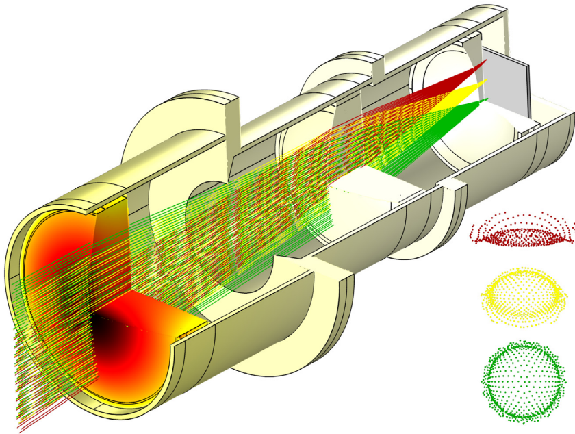
Figure 2-6: Structural-thermal-optical-performance (STOP) analysis of a Petzval lens assembly. The rays are colored according to their initial field angle. Spot diagrams are shown to the right of the main plot.
