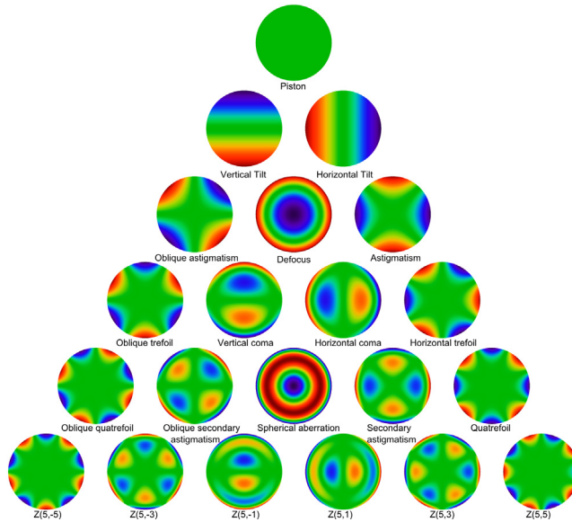
Figure 3-9: Zernike polynomials on the unit circle.
