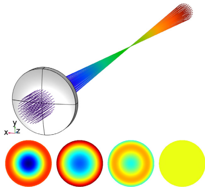
Figure 2-7: Ray trajectories through a simple plano-convex lens (top) and the resulting monochromatic aberrations (bottom). Zernike polynomials: sum of all terms (far left), defocus (left), spherical aberration (right), and all other terms (far right).
