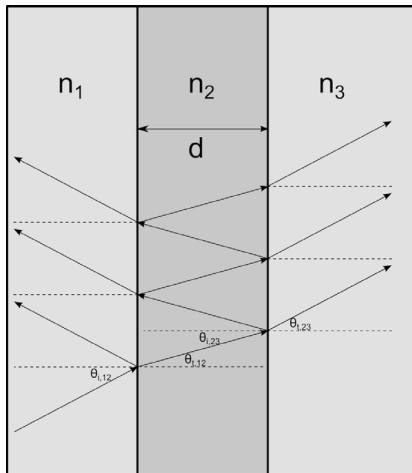
Figure 3-8: One incident ray enters a thin dielectric film and produces a large number of coherent reflected and refracted rays in the adjacent semi-infinite media. These rays can interfere constructively or destructively with each other.
