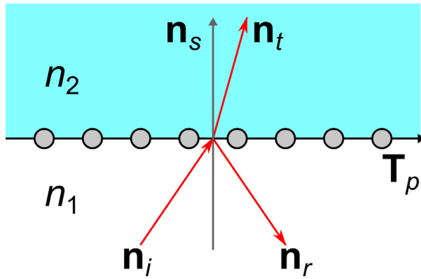
Figure 3-4: Diagram of diffraction grating orientation in 2D.
