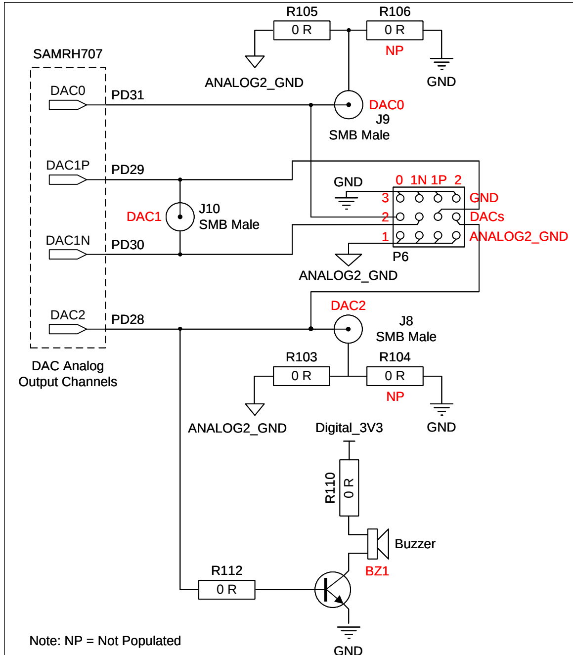
Figure 3-7. DAC Analog Output Channels
