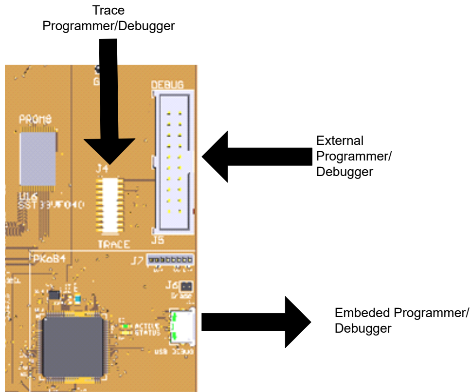
Figure 2-1. Debugging Resources
