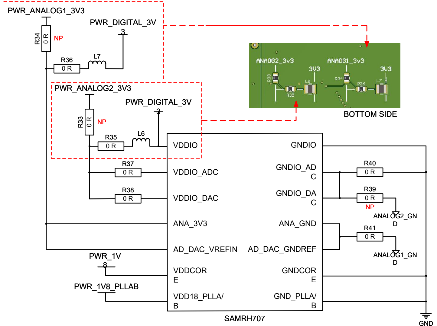
Figure 3-2. Microcontroller Power Supplies
