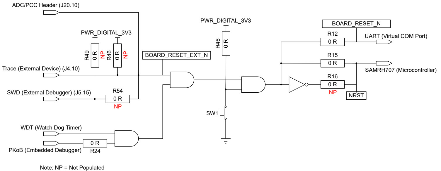
Figure 3-4. Reset Network
