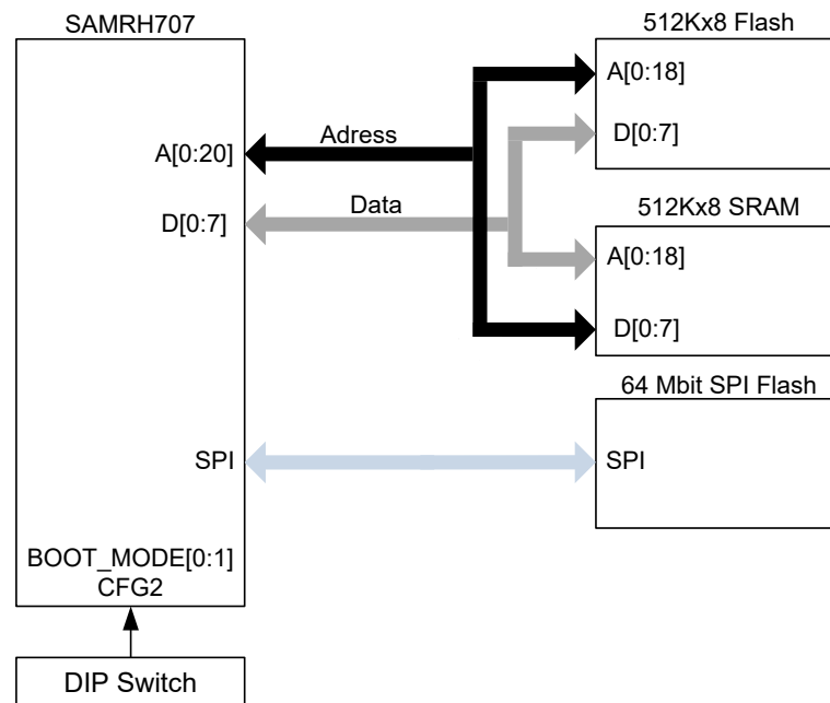
Figure 3-5. Memory Structure
