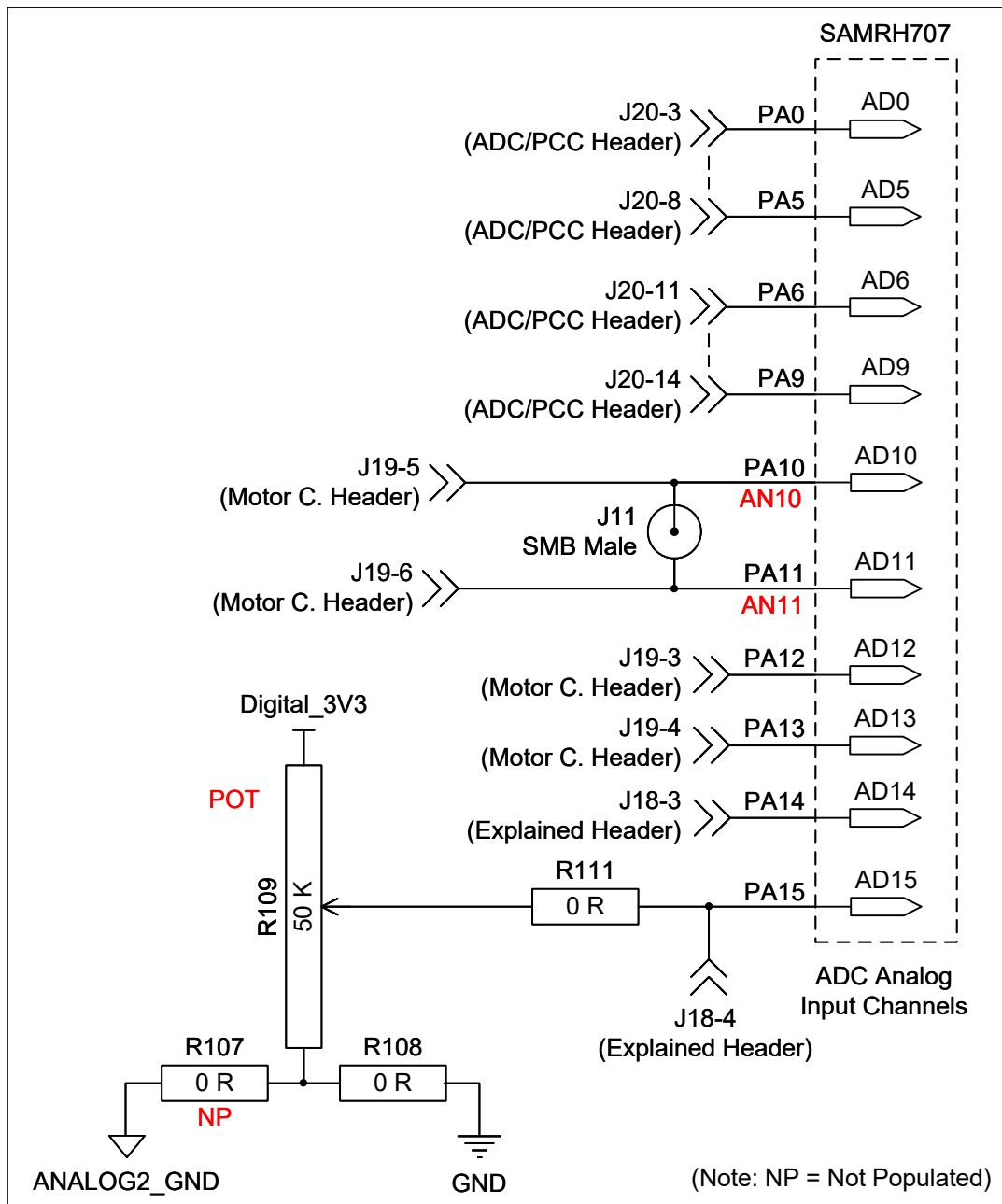
Figure 3-6. ADC Analog Input Channels
