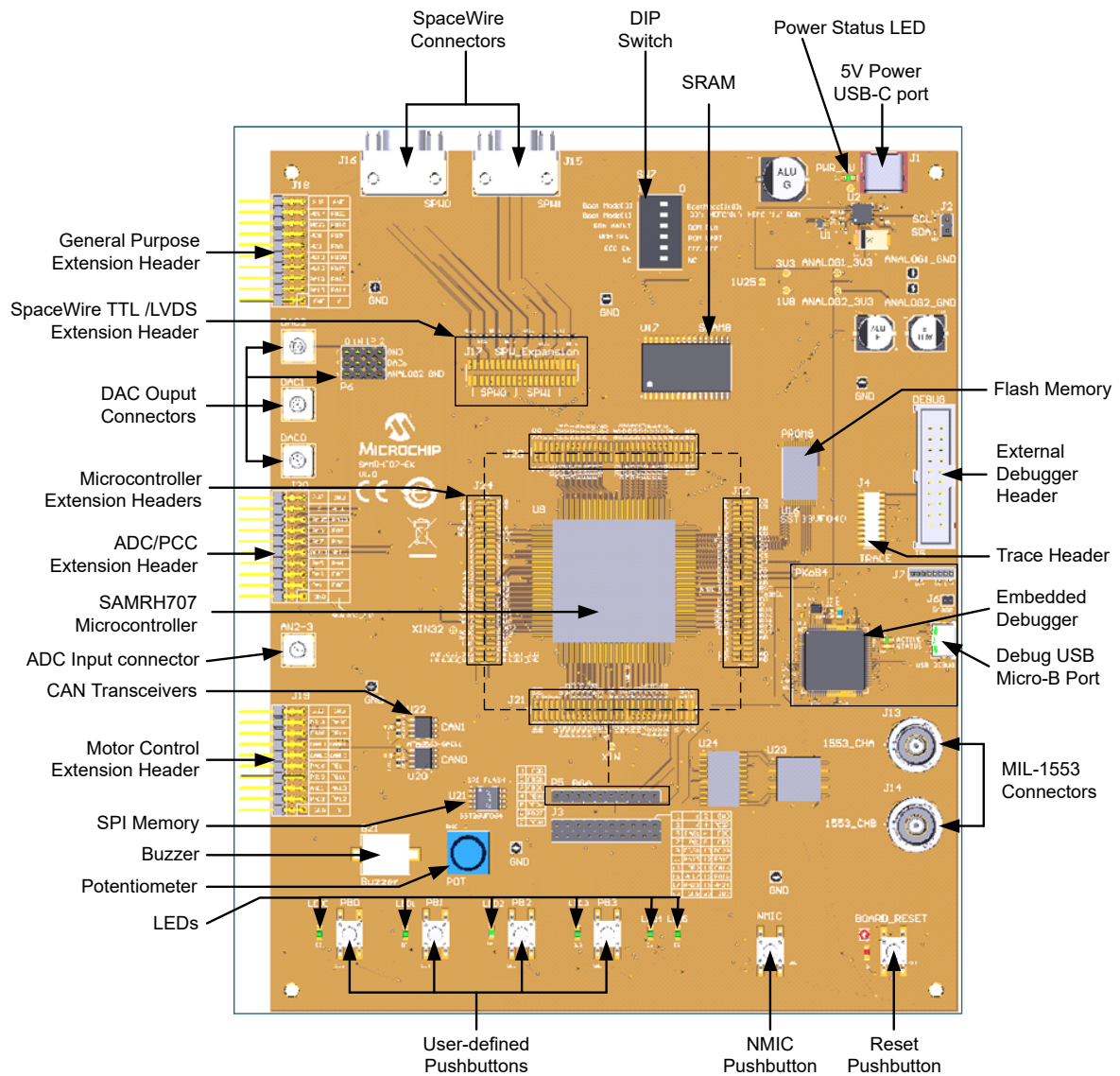
Figure 1-1. SAMRH707F18-EK Board Layout
