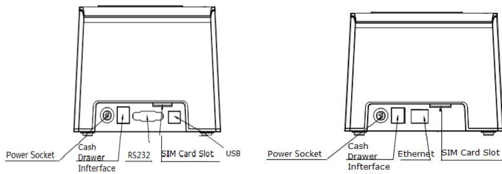
Figure 2-1 Printer Part Name Diagram
