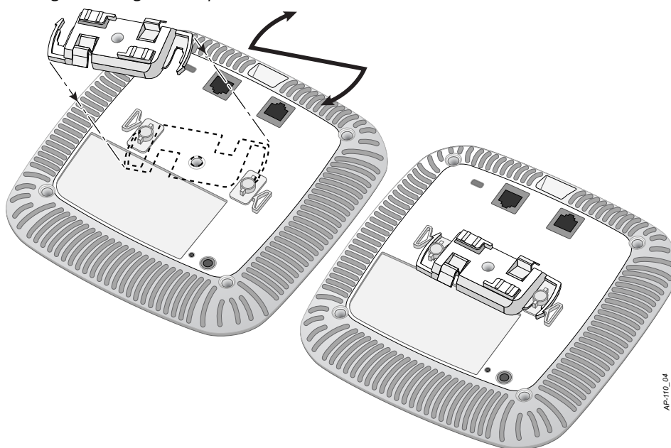
Figure 7 Attaching the Ceiling Rail Adapter
