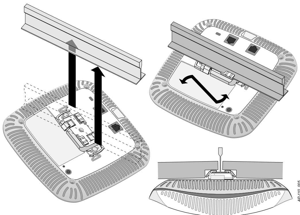
Figure 8 Mounting the AP
