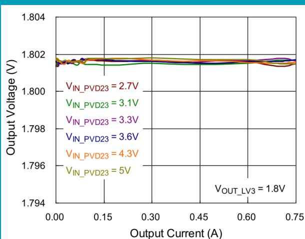
BUCK3 Load Regulation
