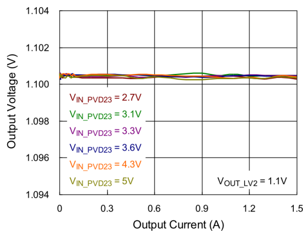
BUCK3 Load Regulation
