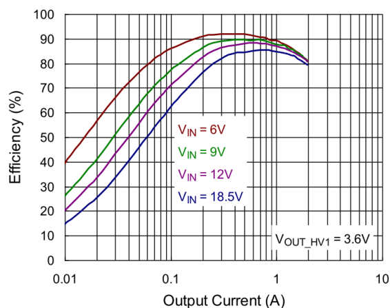
BUCK2 Efficiency
