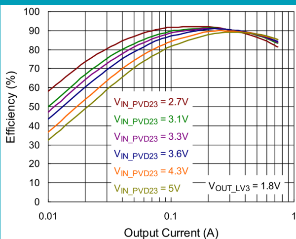
BUCK3 Efficiency
