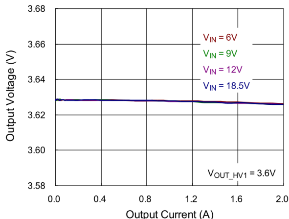
BUCK2 Load Regulation
