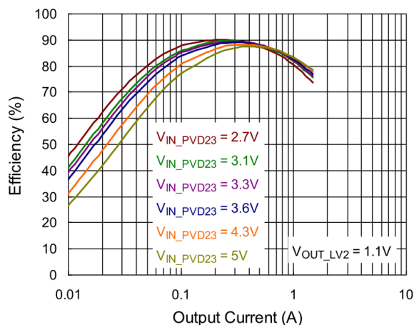
BUCK3 Efficiency
